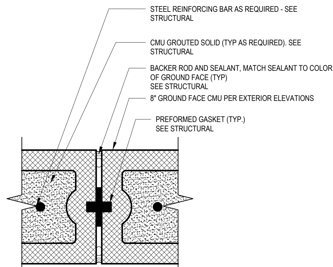
C6 CONTROL JOINT DETAIL 3" = 1'-0"
