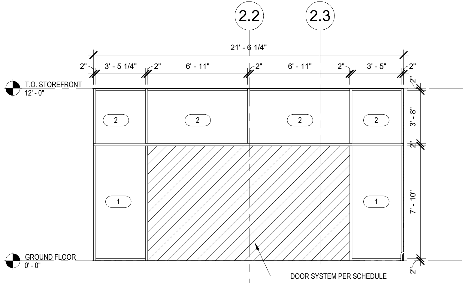
C7 STOREFRONT GLAZING - WINDOW 'B' 1/4" = 1'-0"
