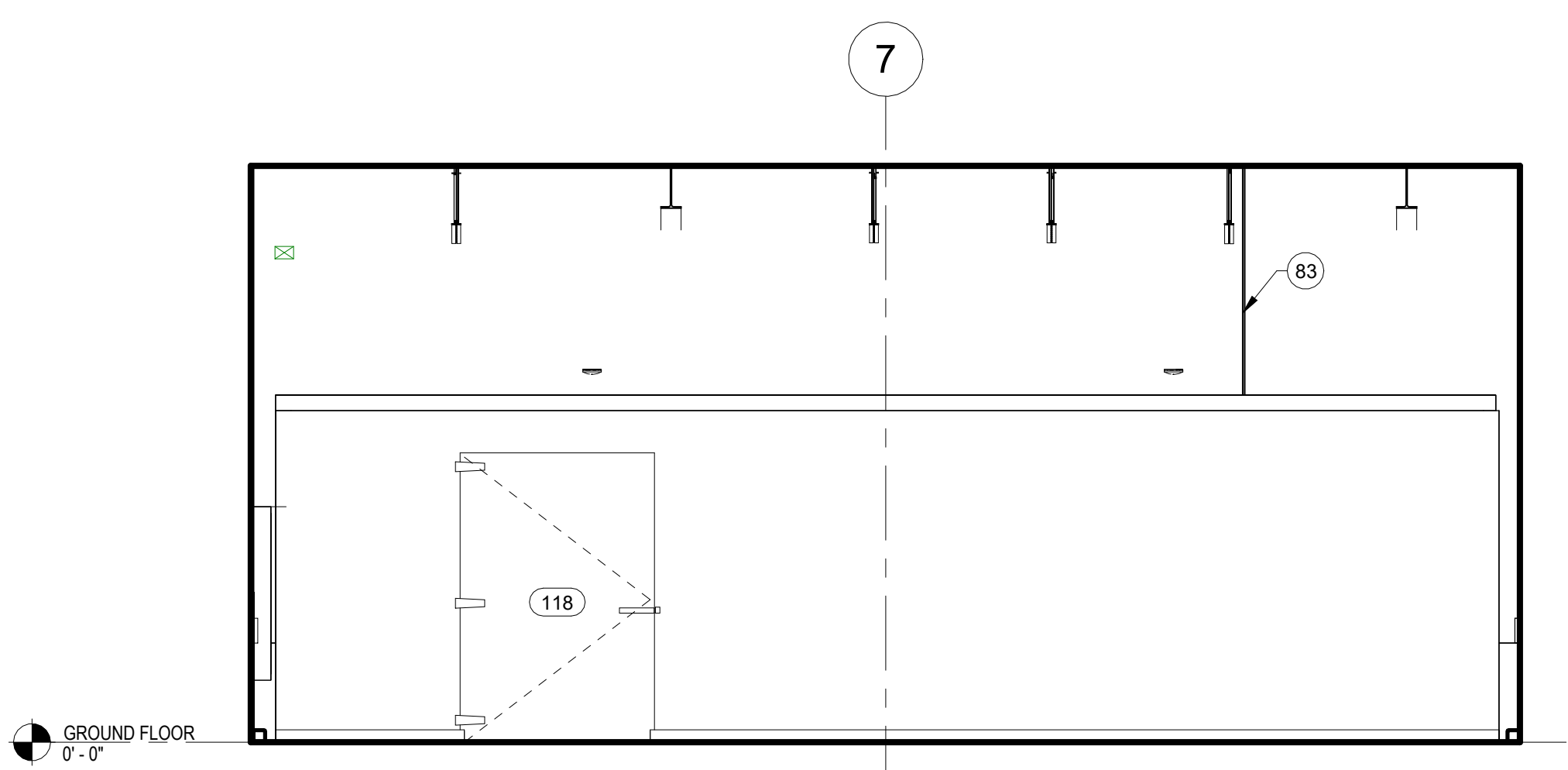
1 INTERIOR ELEVATION - LOADING DOCK 1/4" = 1'-0"
