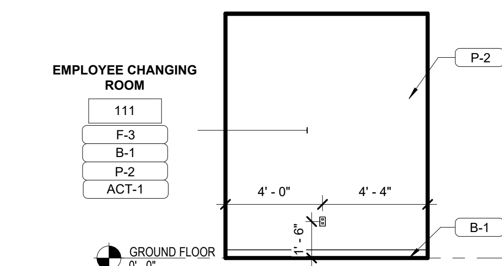
D1 INTERIOR ELEVATION - CHANGING 1/4" = 1'-0"
