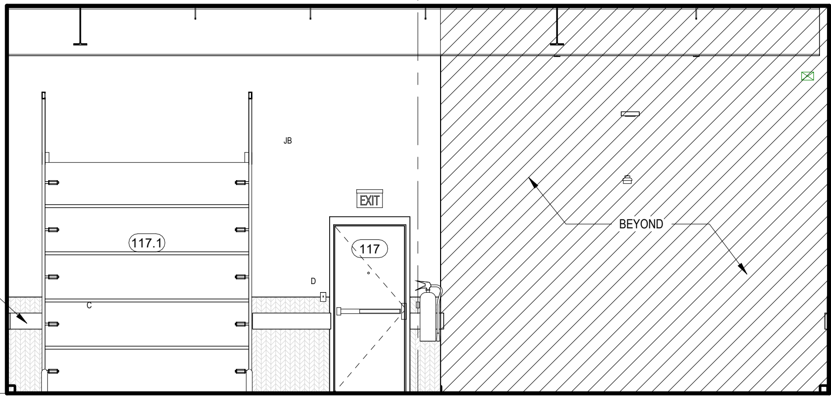
2 INTERIOR ELEVATION - LOADING DOCK 1/4" = 1'-0"
