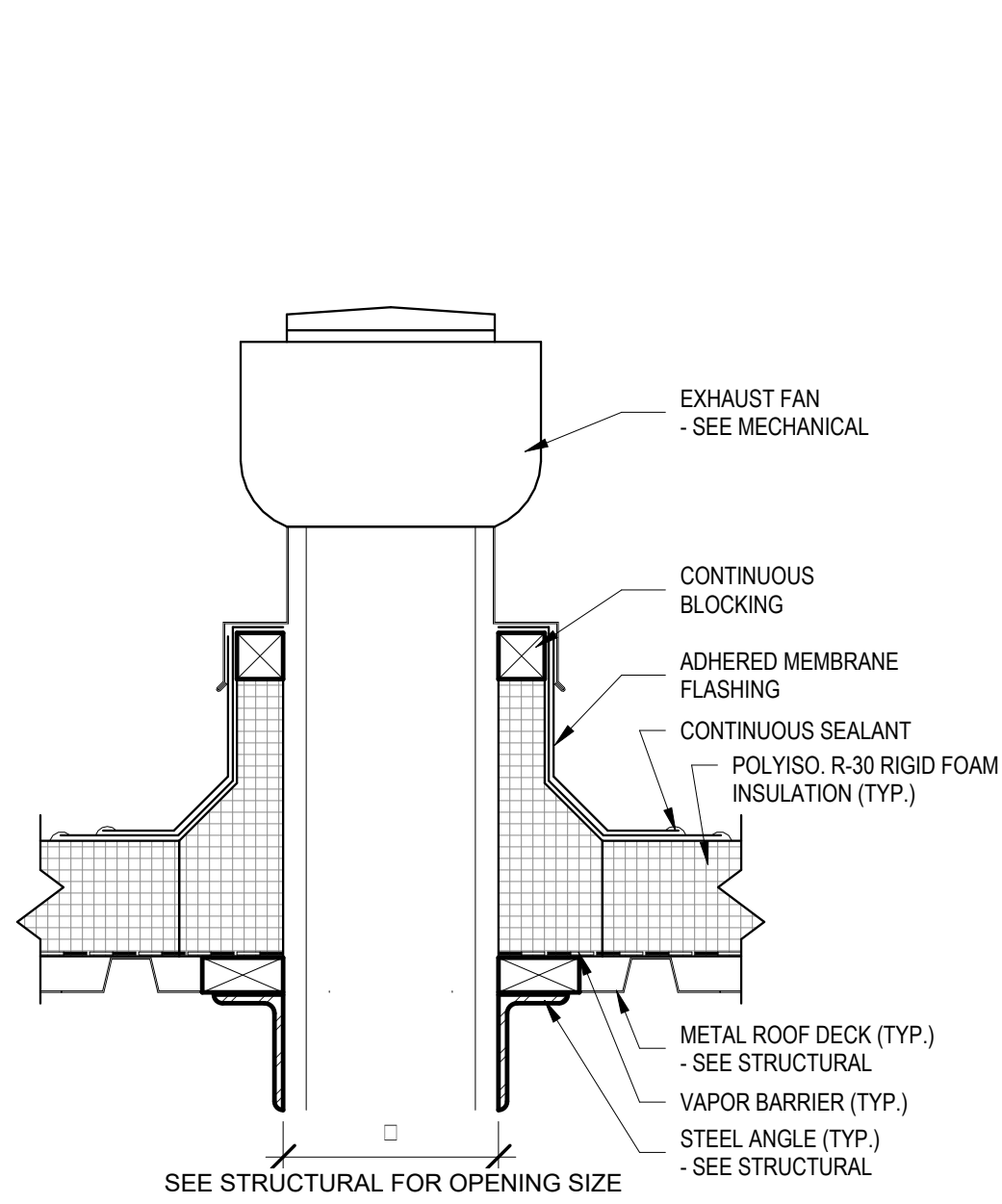
B7 EXHAUST FAN PENETRATION (TYP.) 1 1/2" = 1'-0"
