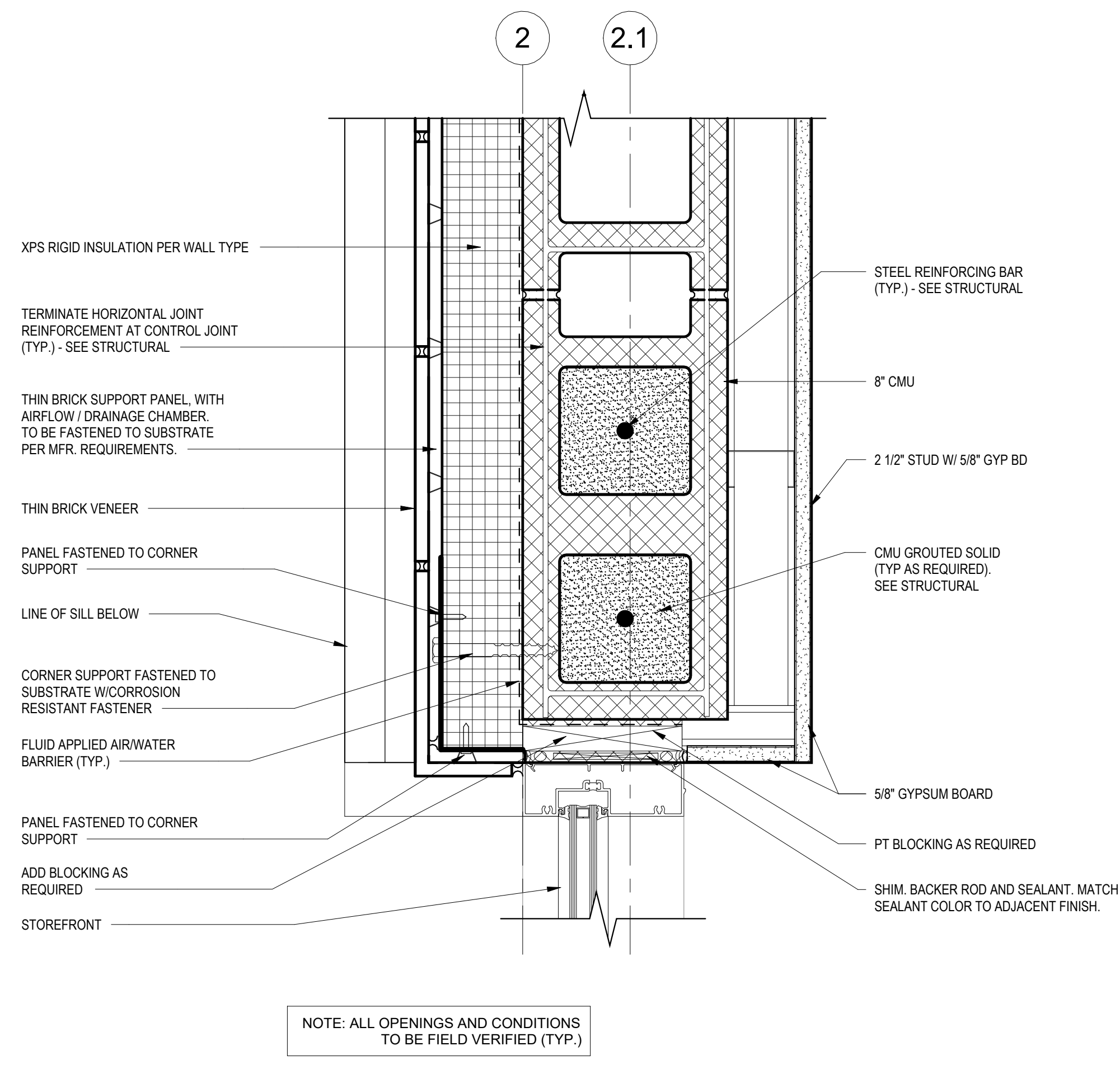
INSIDE CORNER AT COLUMN LINE 2 -ABOVE WATER TABLE E2 3" = 1'-0"
