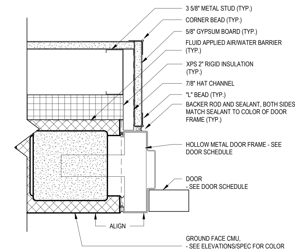
D4 EXTERIOR DOOR JAMB DETAIL - GROUND FACE CMU 3" = 1'-0"
