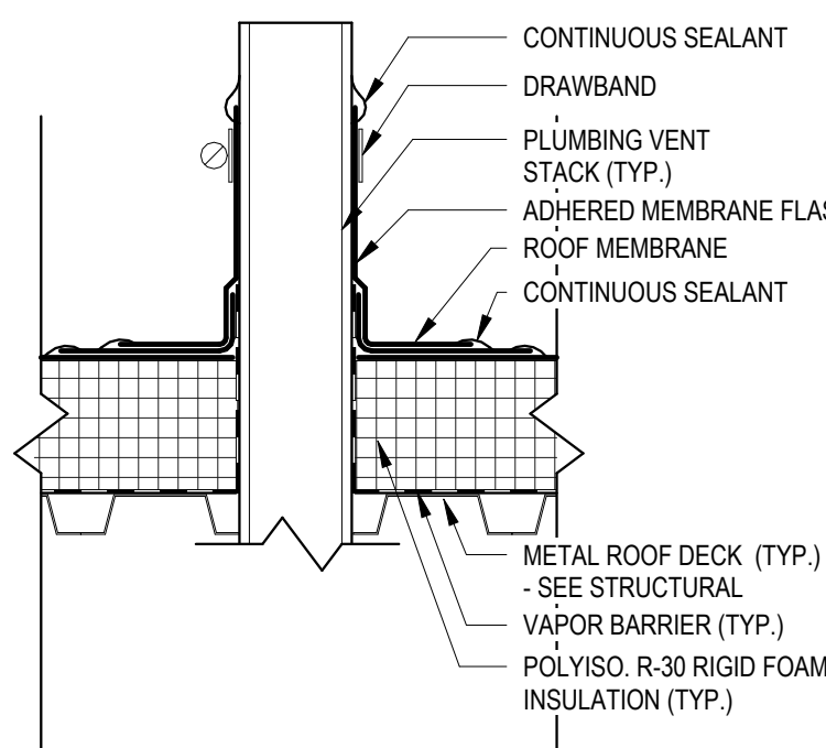
C7 VENT PENETRATION (TYP.) 1 1/2" = 1'-0"
