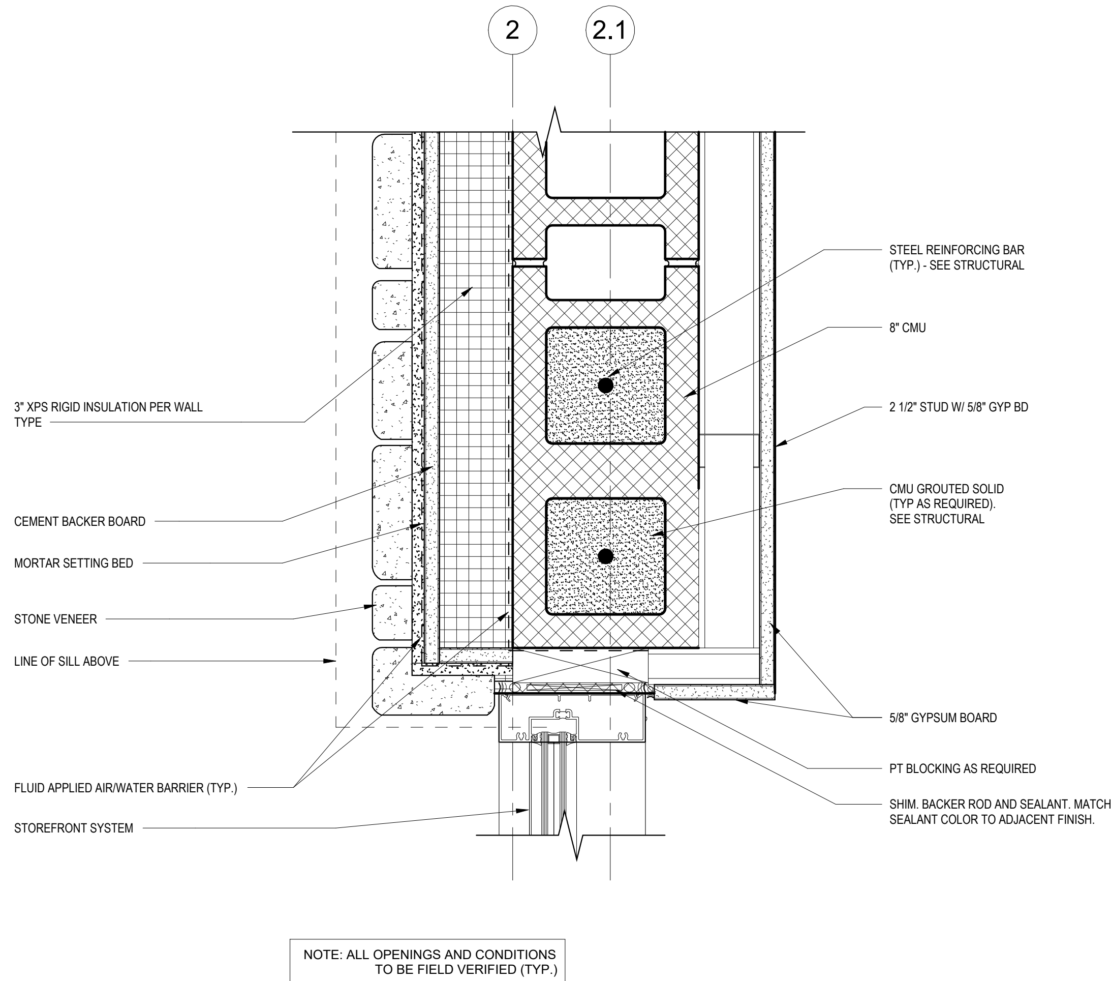
INSIDE CORNER AT COLUMN LINE 2 -BELOW WATER TABLE E6 3" = 1'-0"
