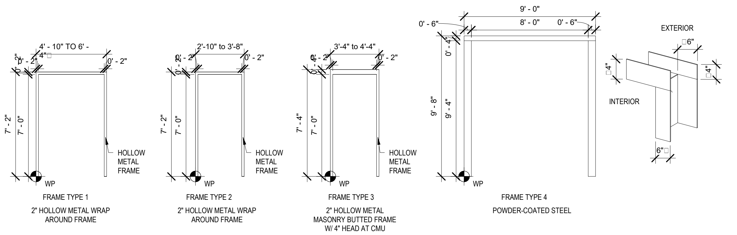
D2 FRAME ELEVATIONS 1/4" = 1'-0"
