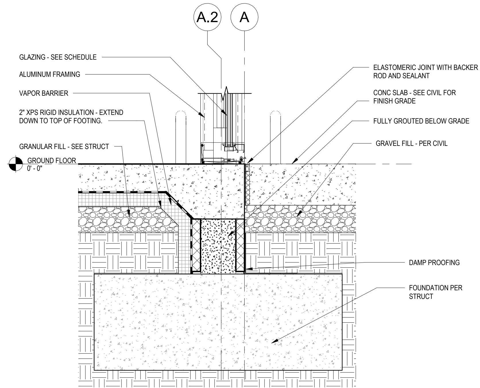
B6 FOUNDATION AT ENTRY STOREFRONT 1 1/2" = 1'-0"
