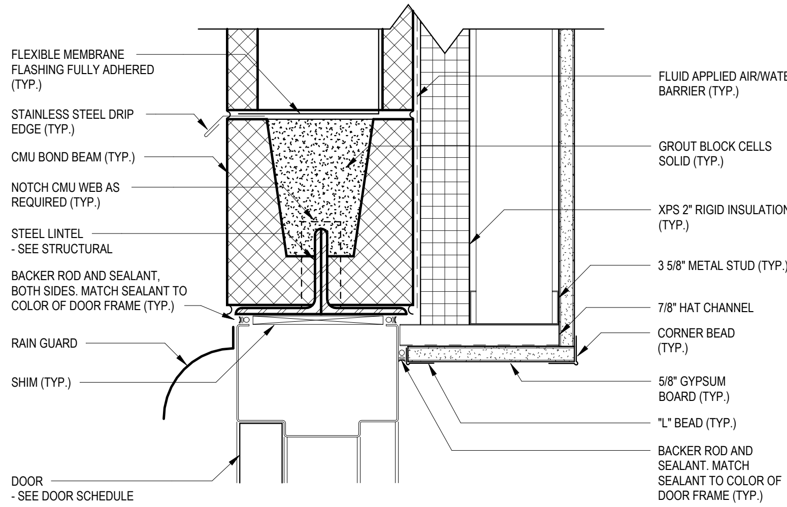
C4 EXTERIOR DOOR HEAD DETAIL - GROUND FACE CMU 3" = 1'-0"
