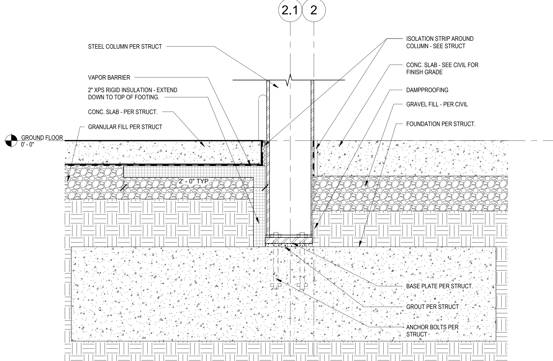
B4 FOUNDATION AT COLUMN 1 1/2" = 1'-0"
