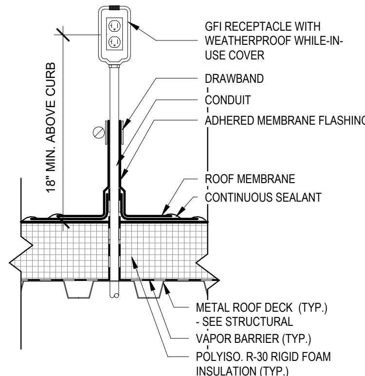
C4 ROOFTOP RECEPTACLE (TYP.) 1 1/2" = 1'-0"
