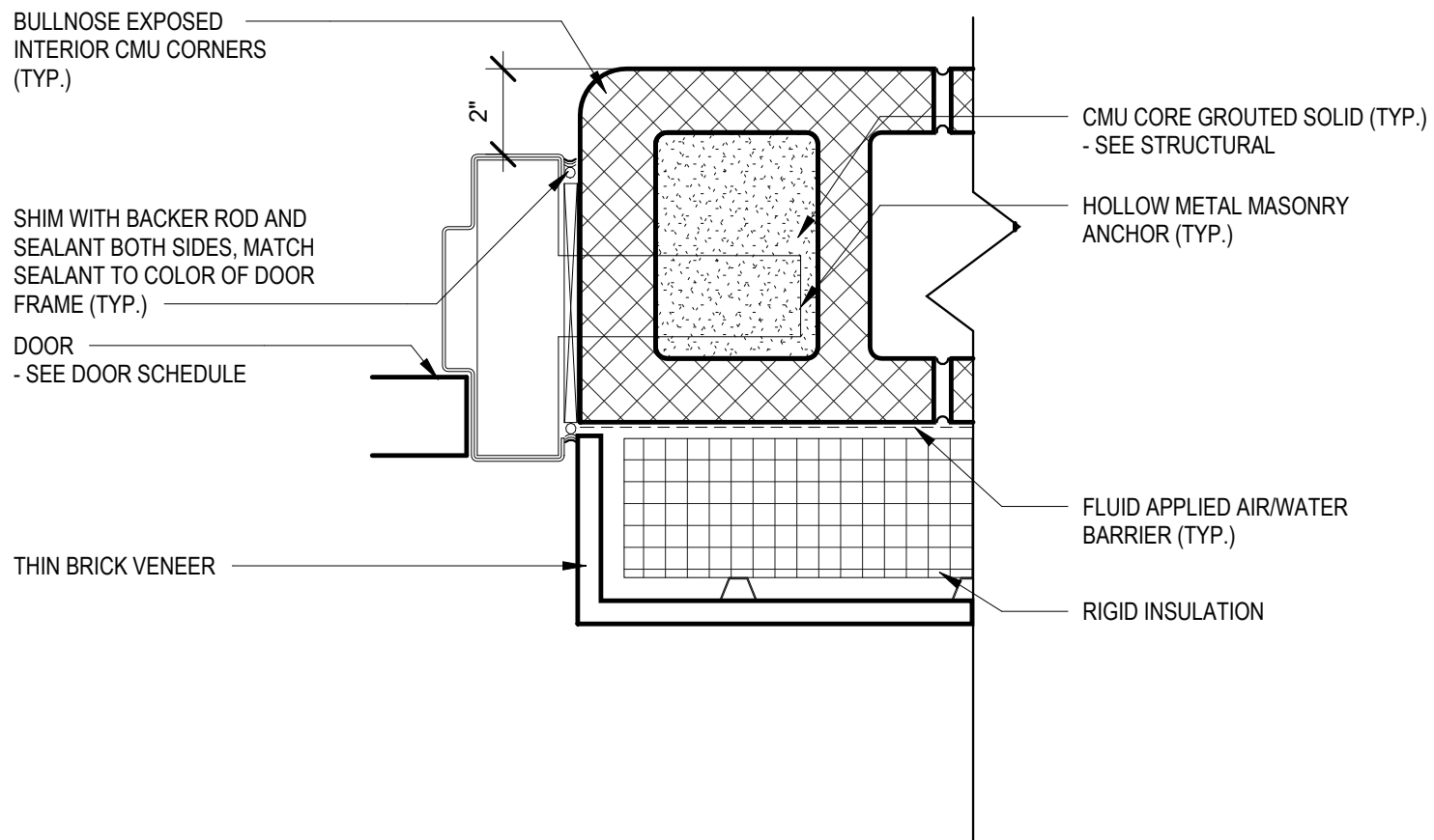
C2 EXTERIOR DOOR JAMB DETAIL - ABOVE SILL 3" = 1'-0"
