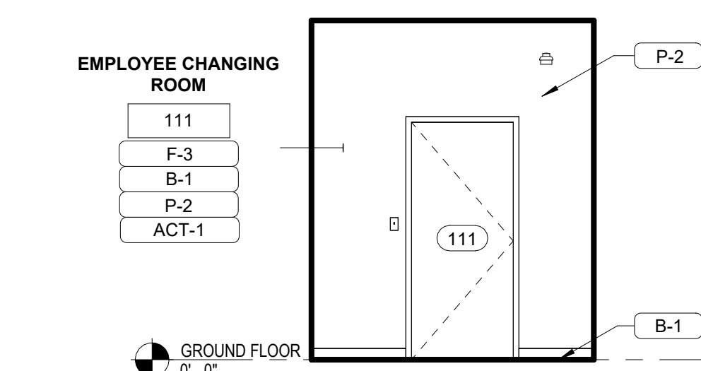
C1 INTERIOR ELEVATION - CHANGING 1/4" = 1'-0"
