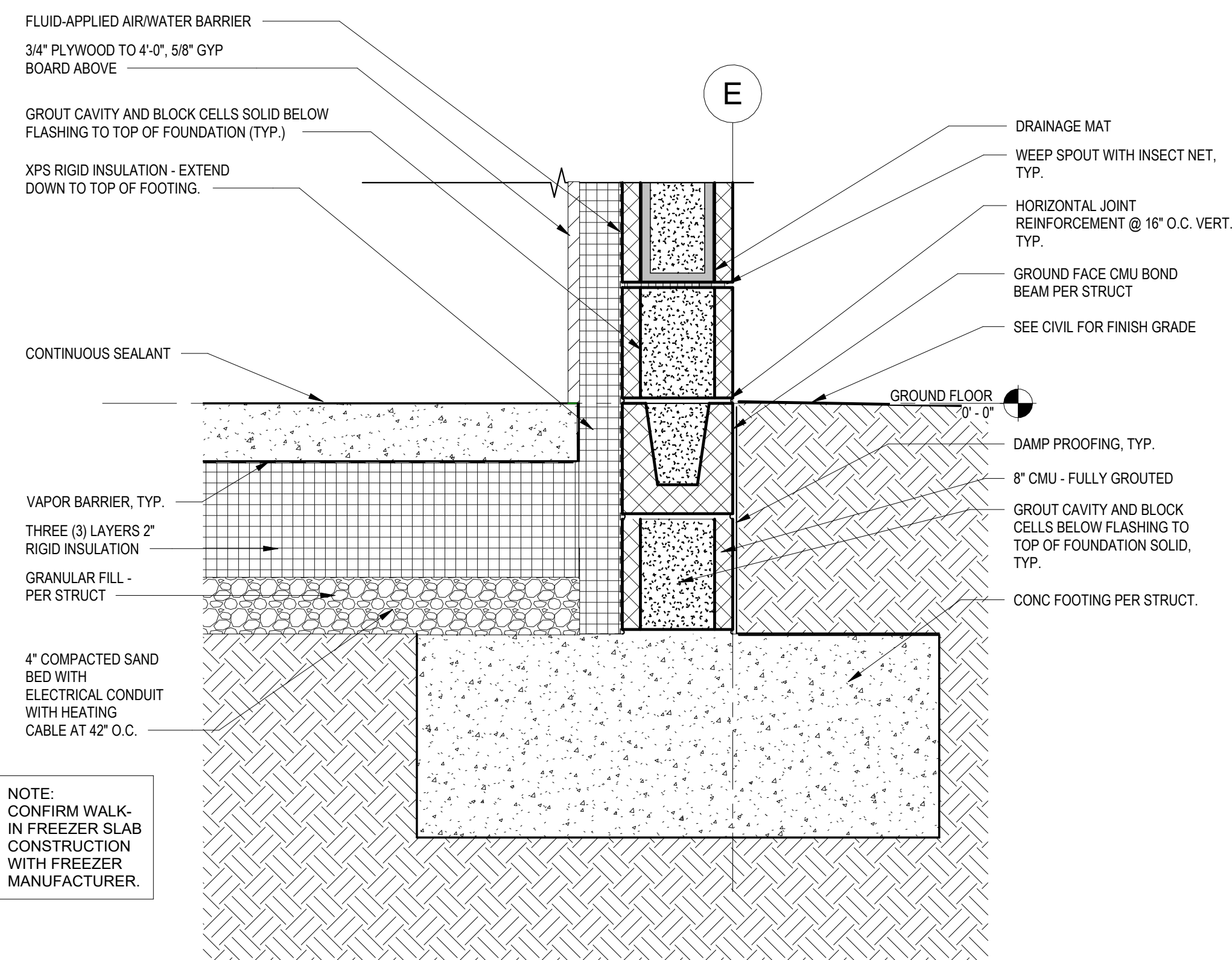
C6 FOUNDATION AT COOLER 1 1/2" = 1'-0"
