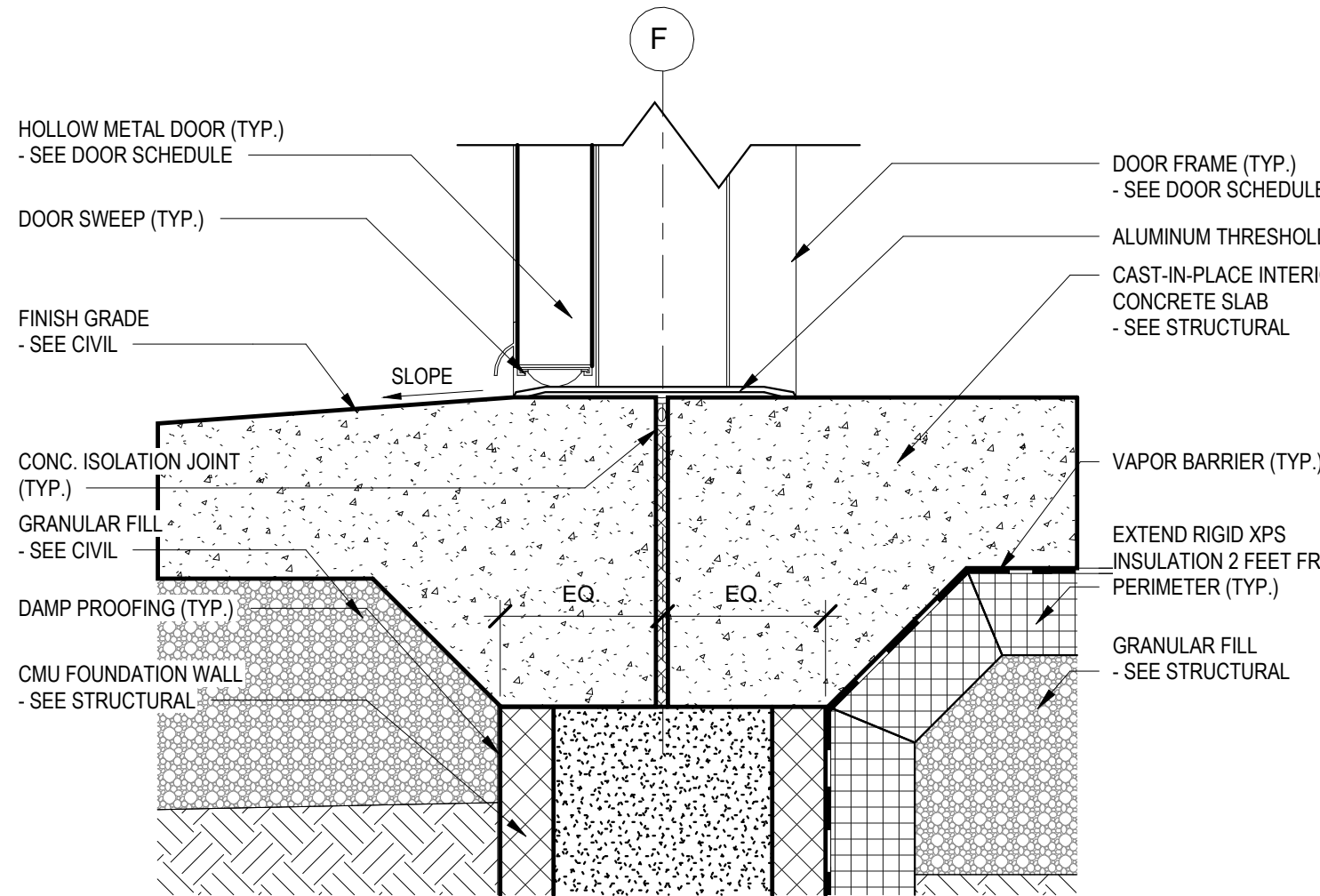
E4 EXTERIOR DOOR SILL DETAIL 3" = 1'-0"
