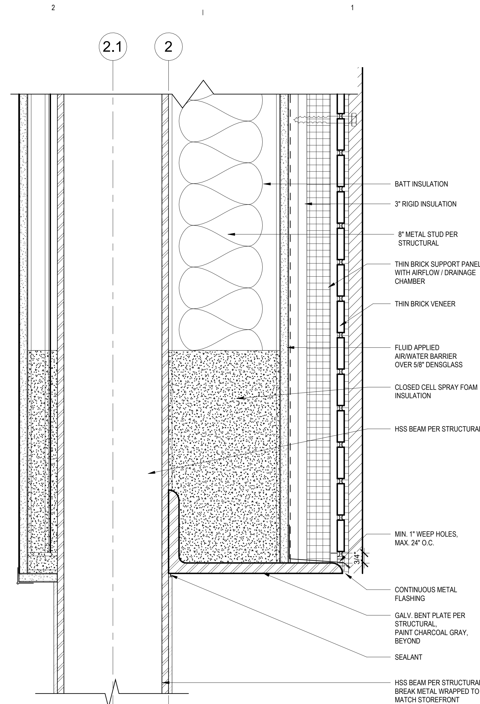
C2 COLUMN TO WALL CONNECTION AT BRICK/METAL STUD 3" = 1'-0"
