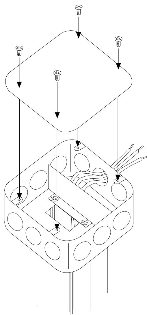
E1 TPB GASKETED BOX 1/2" = 1'-0"
