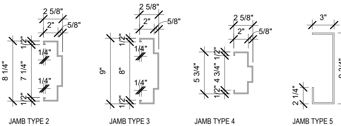
A2 JAMB PROFILES 1 1/2" = 1'-0"
