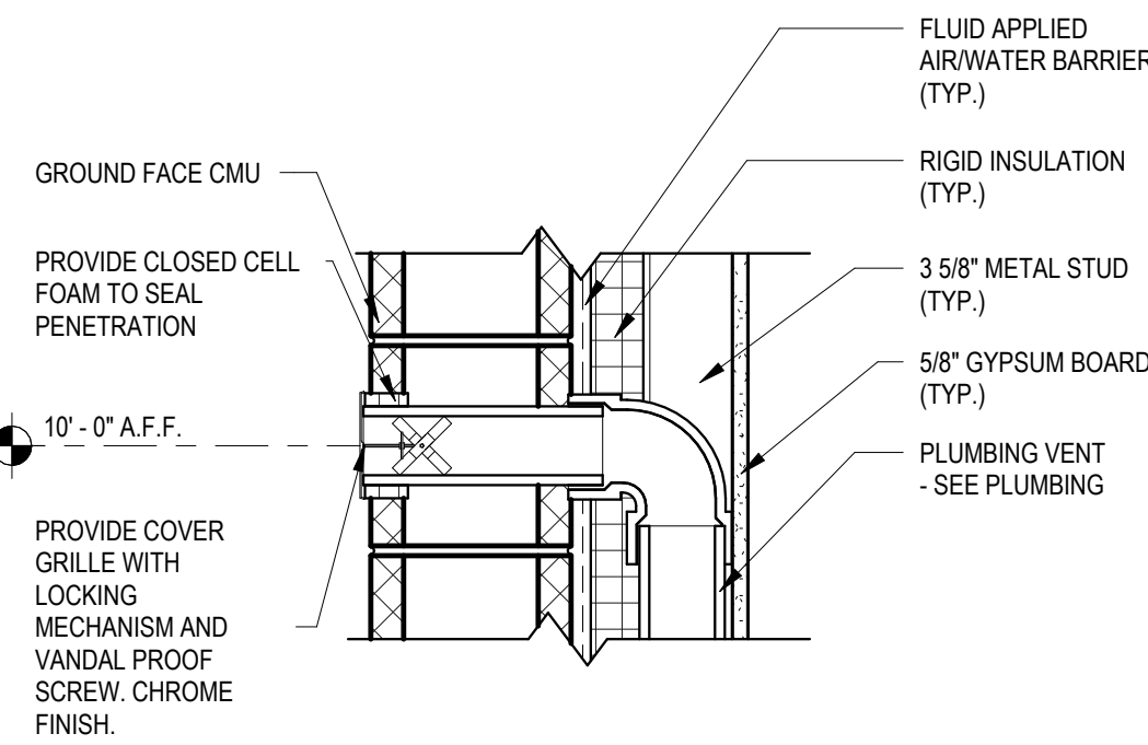
C5 HORIZONTAL VENT (TYP.) 1 1/2" = 1'-0"
