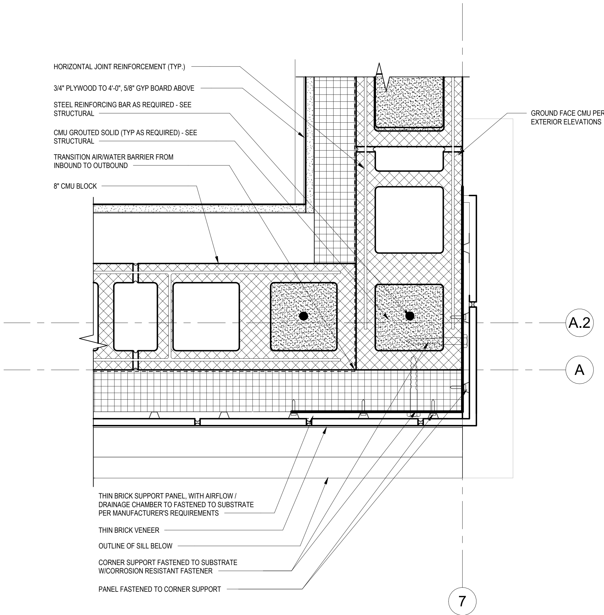
E7 COLUMN LINE A-7 - ABOVE WATER TABLE 3" = 1'-0"
