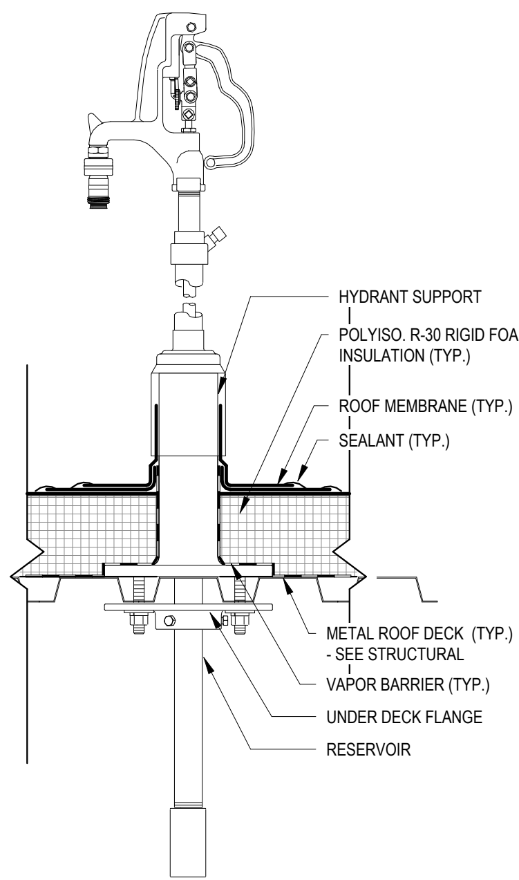
B5 ROOFTOP HOSE BIB 1 1/2" = 1'-0"
