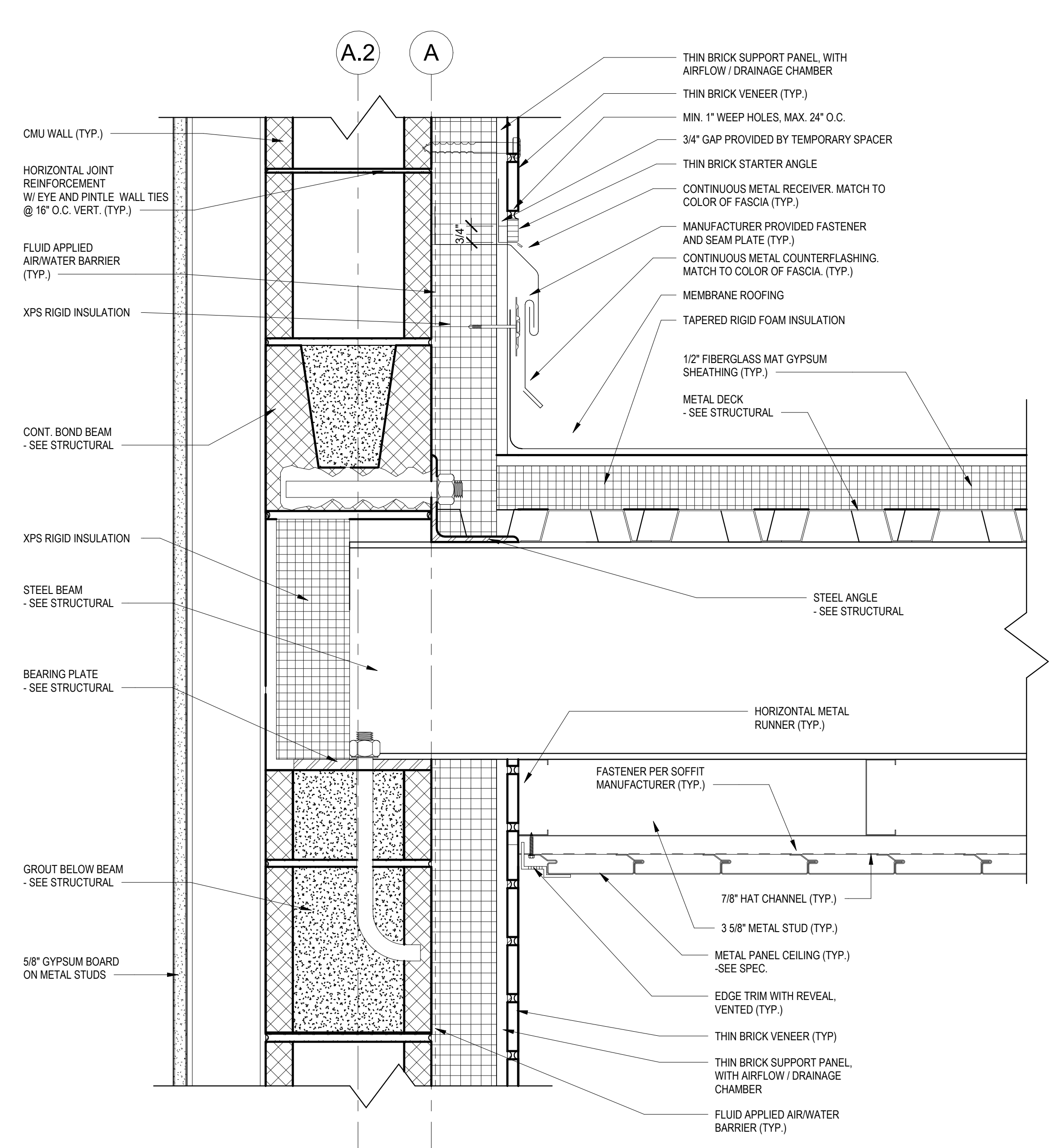
E2 CANOPY @ BRICK/BRICK CMU 3" = 1'-0"
