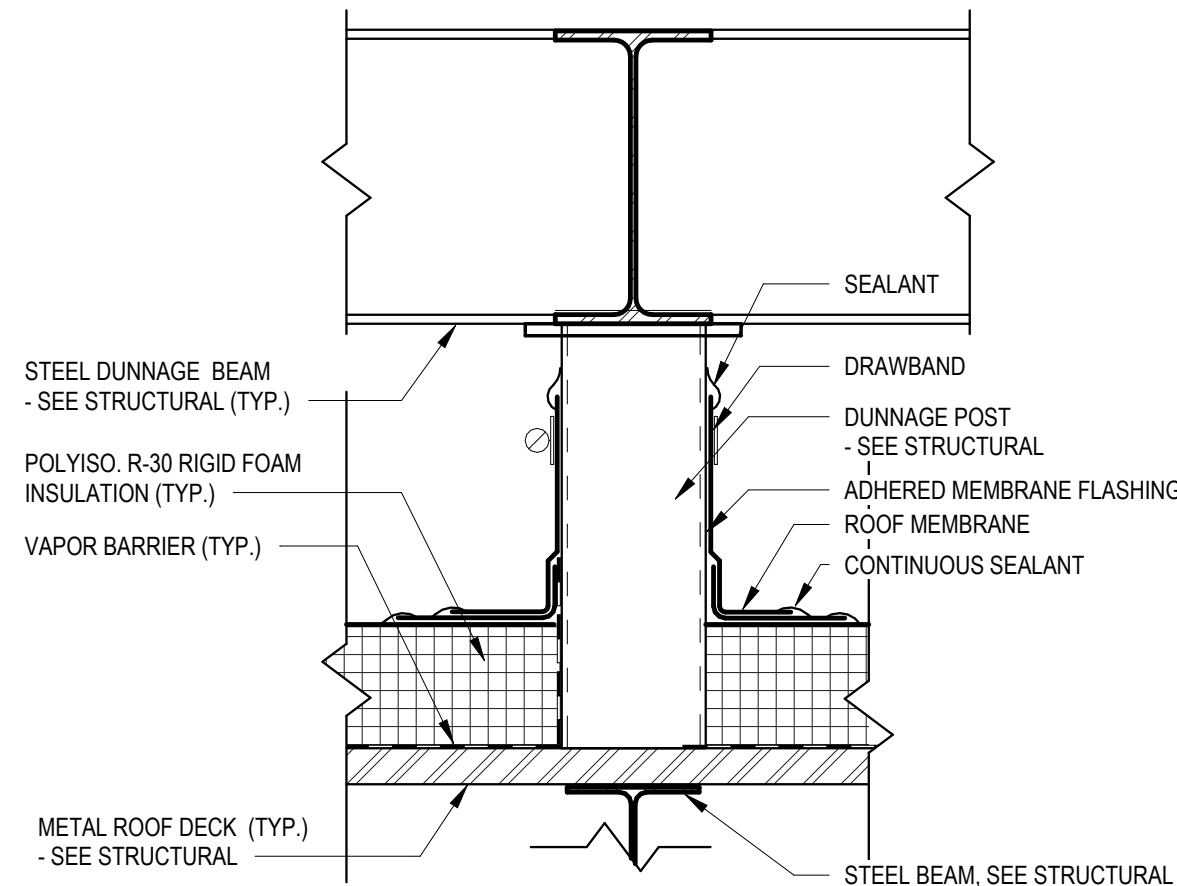
D7 ROOF PENETRATION AT DRY COOLER DUNNAGE 1 1/2" = 1'-0"
