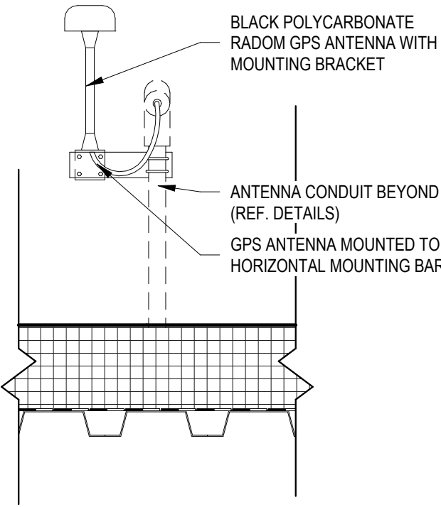
D2 GPS ANTENNA MOUNTING DETAIL (TYP.) 1 1/2" = 1'-0"
