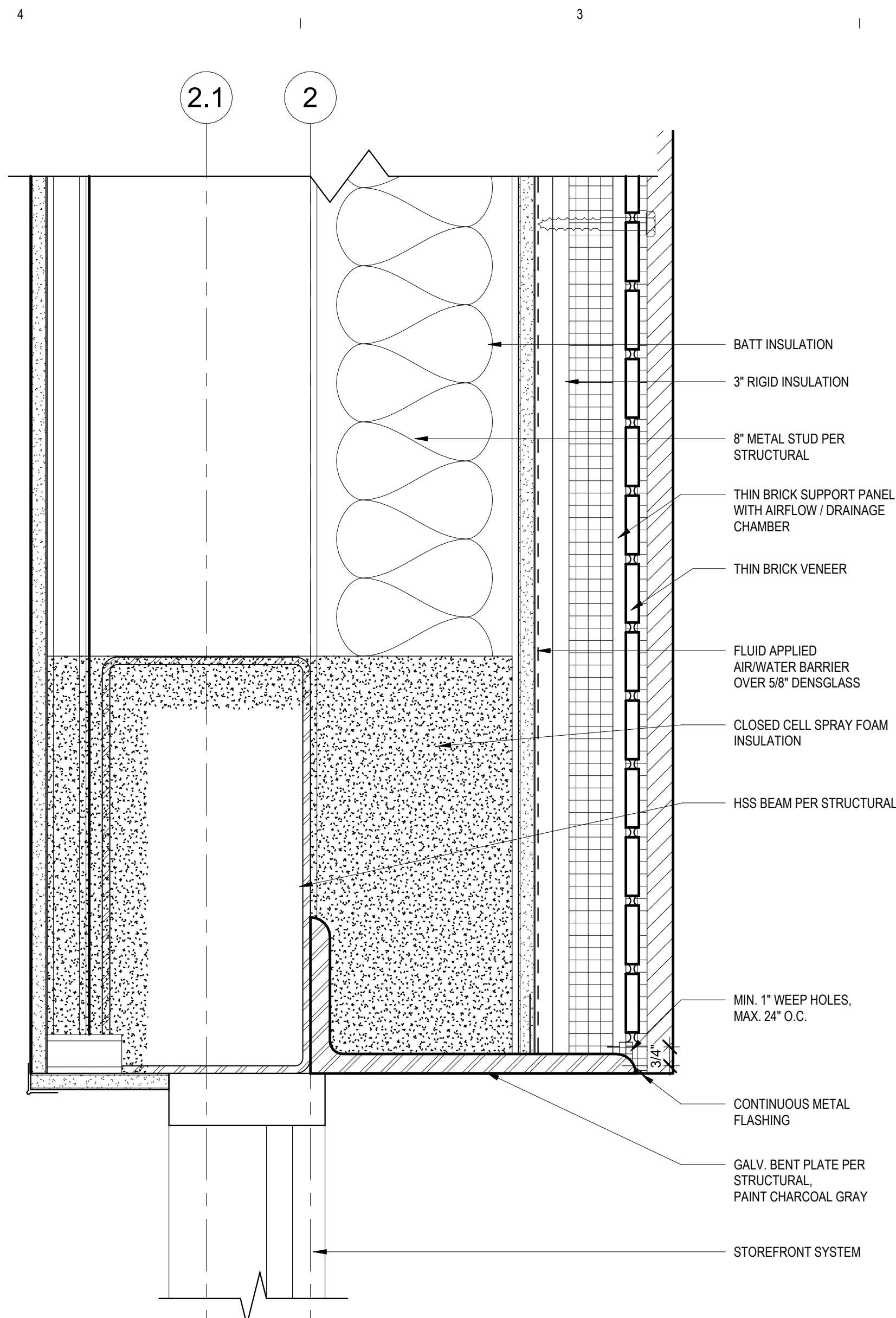
C4 BRICK WALL ABOVE STOREFRONT 3" = 1'-0"
