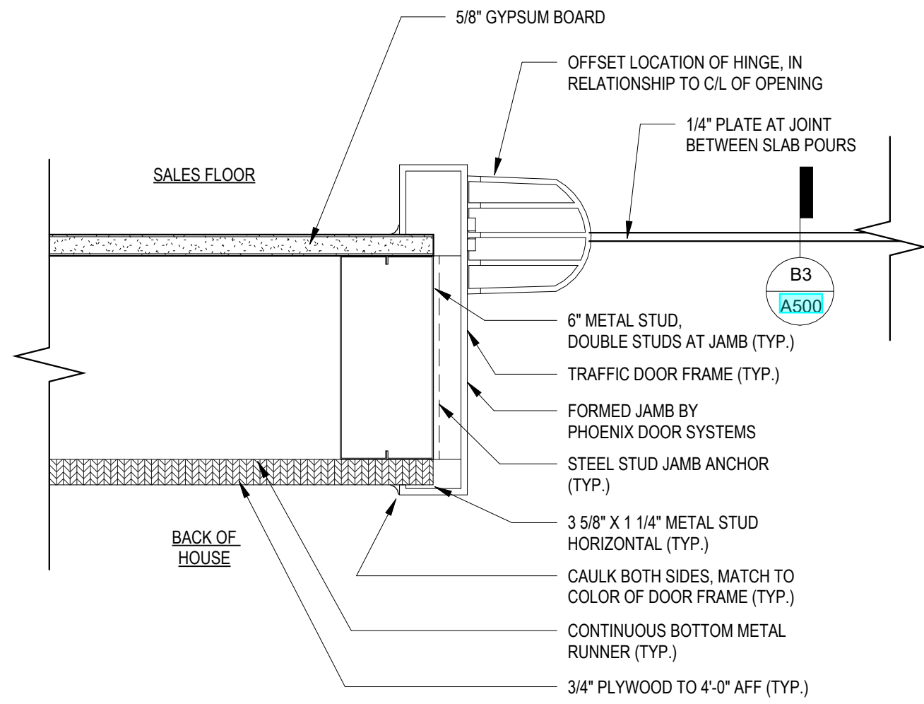
B3 TRAFFIC DOOR JAMB DETAIL - LOW 3" = 1'-0"
