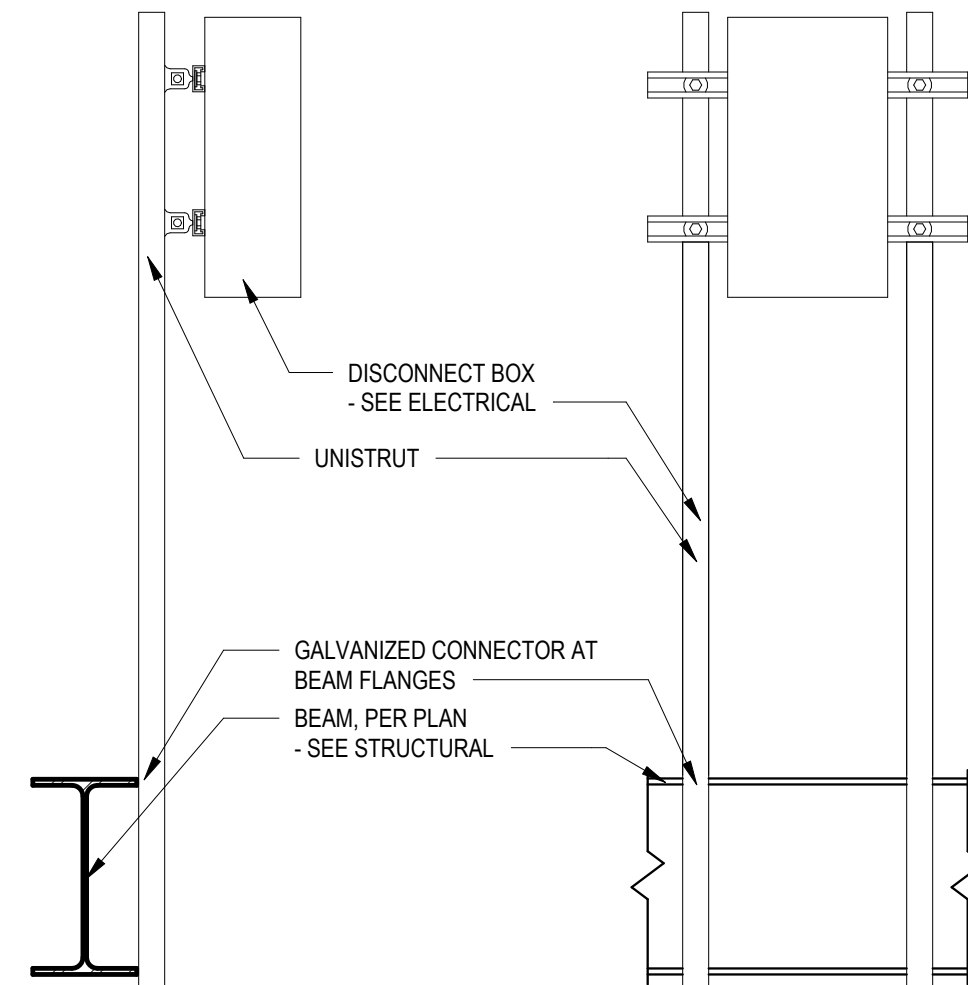
TYP. DRY COOLER DISCONNECT MOUNTING 1" = 1'-0"
