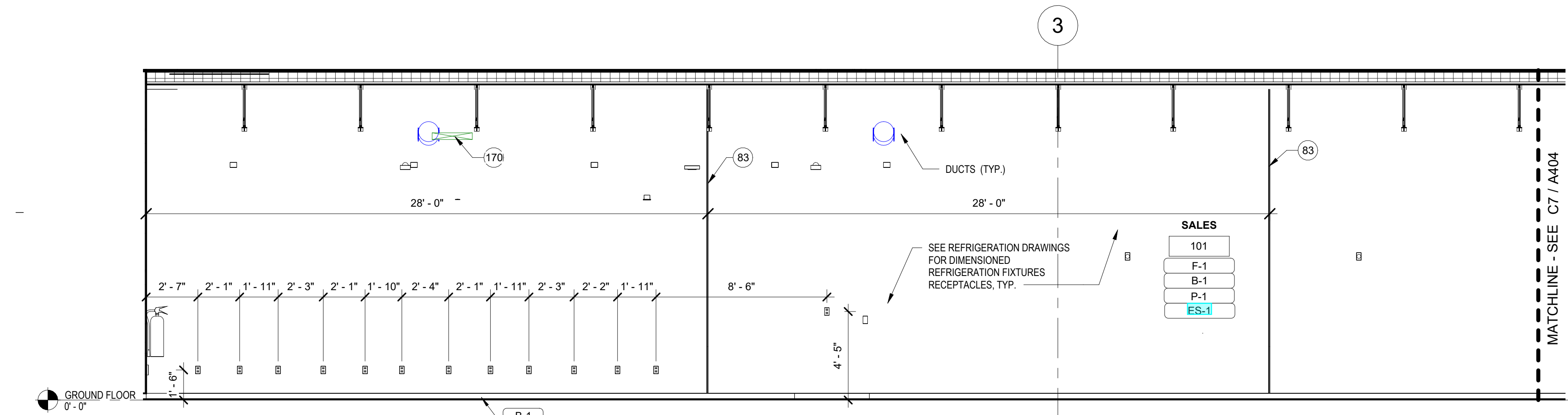
D7 INTERIOR ELEVATION - SALES FLOOR, CONT. 1/4" = 1'-0"
