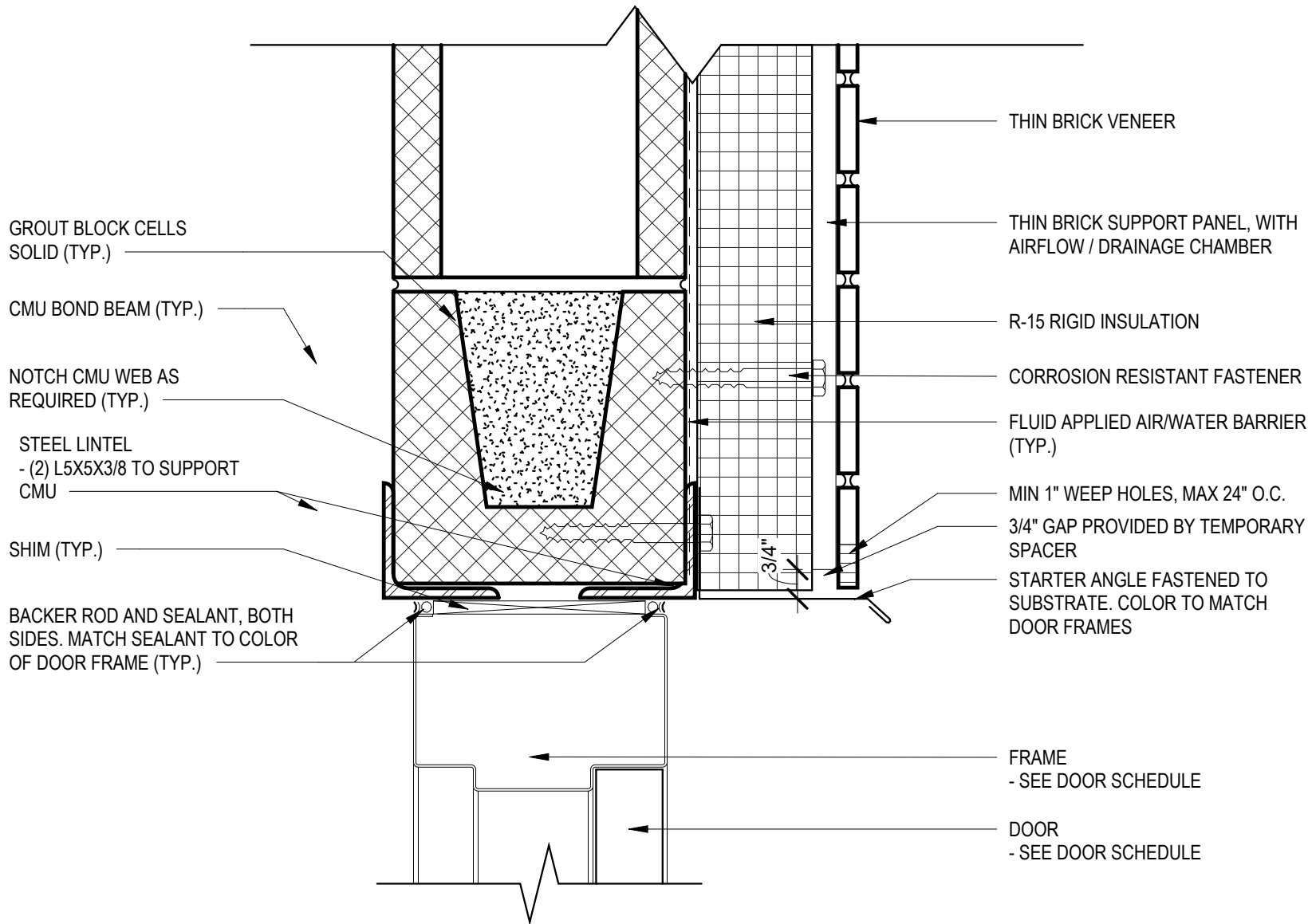
B2 EXTERIOR DOOR HEAD DETAIL IN BRICK 3" = 1'-0"
