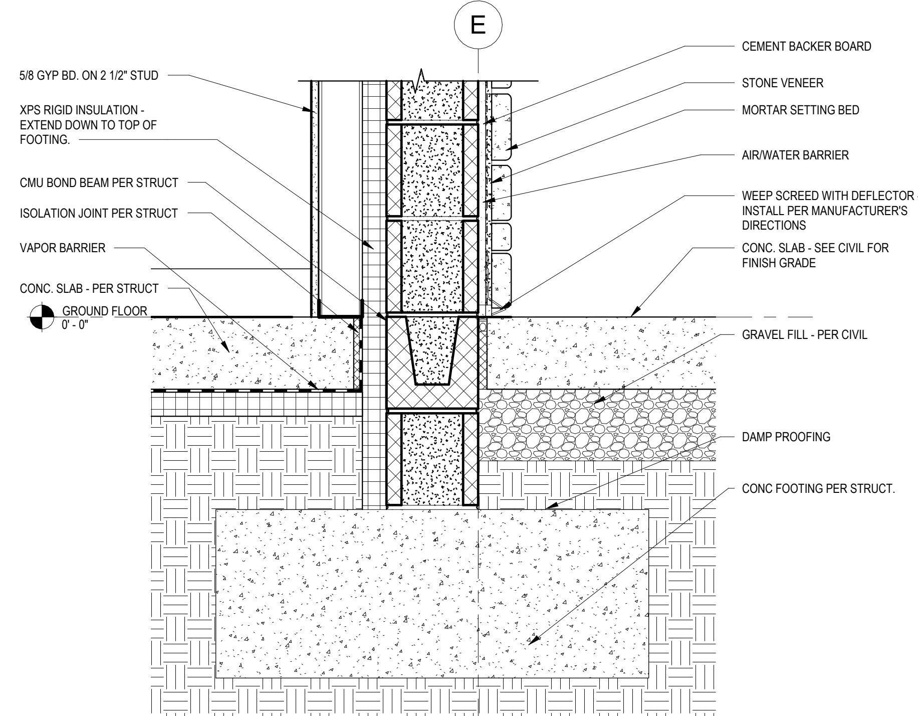
B2 FOUNDATION AT STONE VENEER 1 1/2" = 1'-0"
