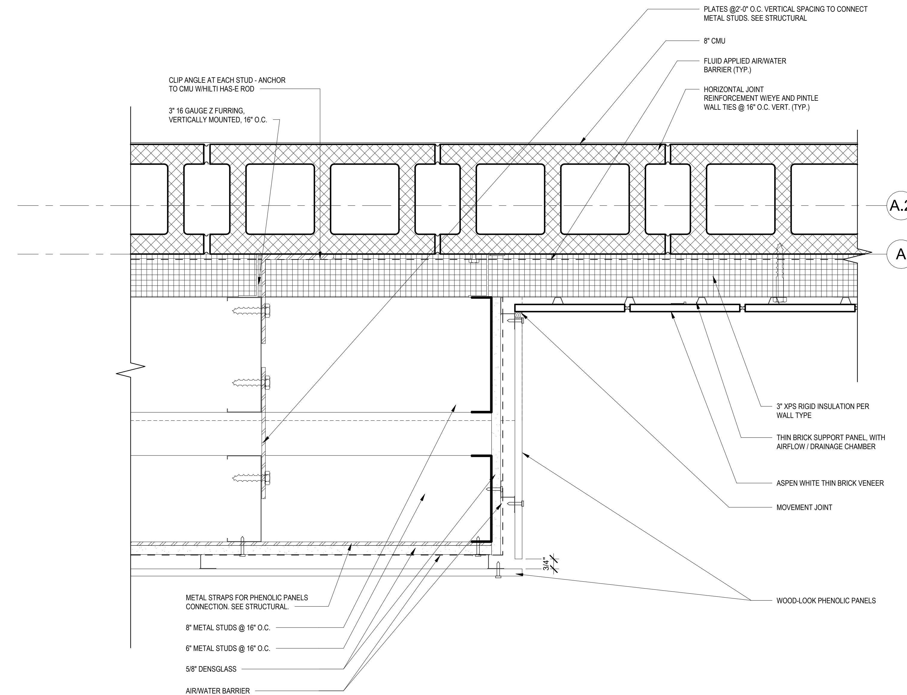
E2 FINISH TRANSITION ABOVE CANOPY 3" = 1'-0"
