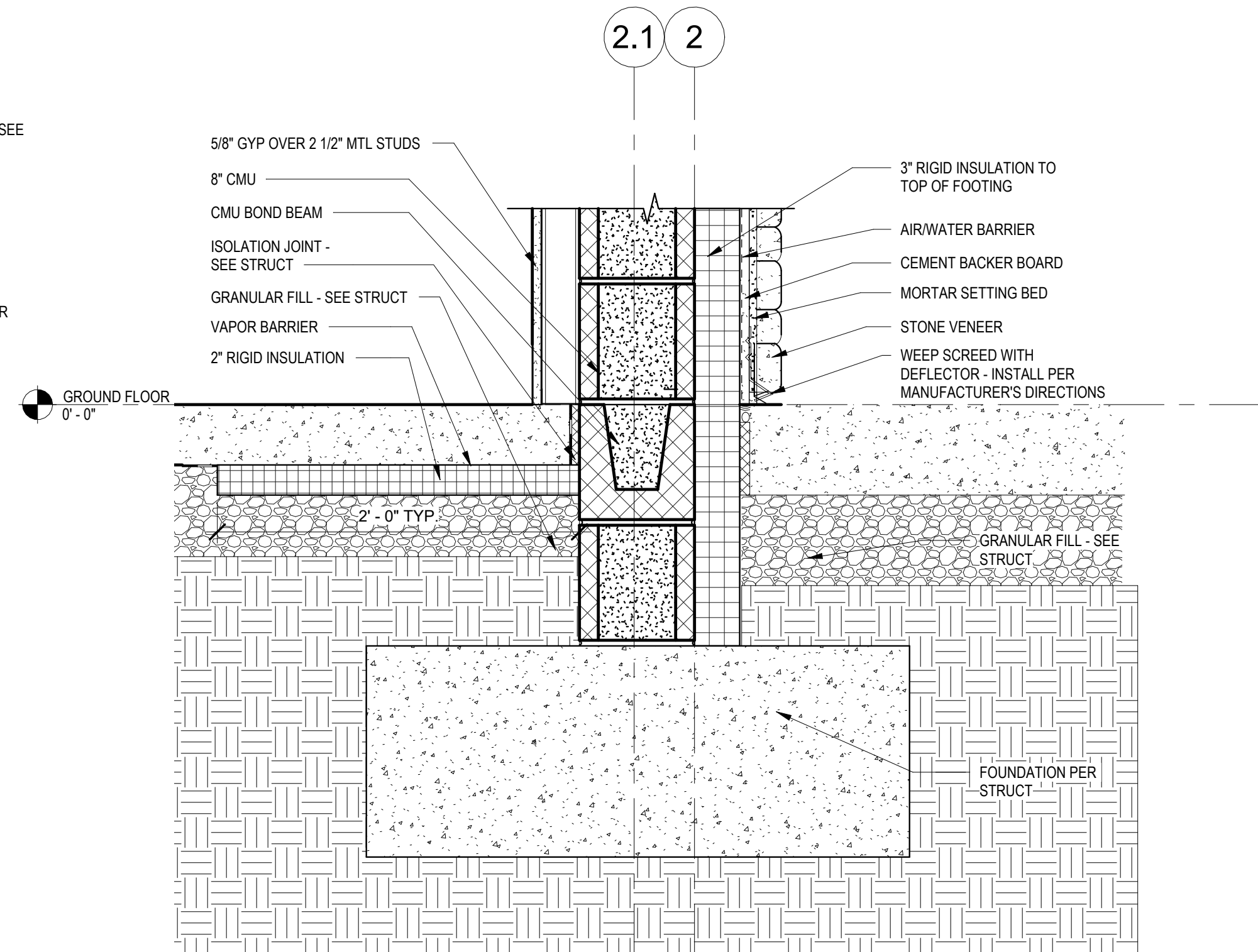
D2 FOUNDATION AT SHEAR WALL 1 1/2" = 1'-0"
