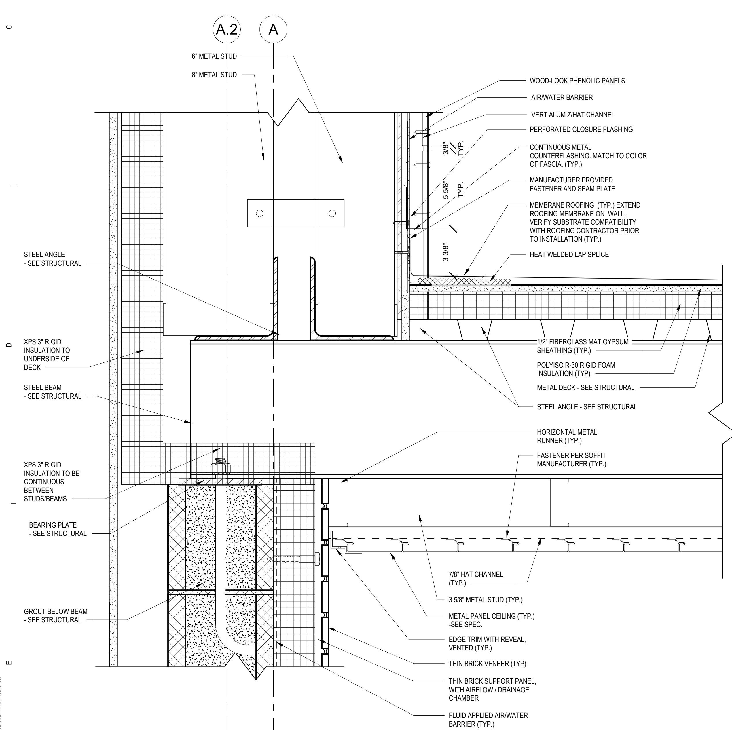
E6 CANOPY @ SIDING/BRICK CMU CONNECTION 3" = 1'-0"
