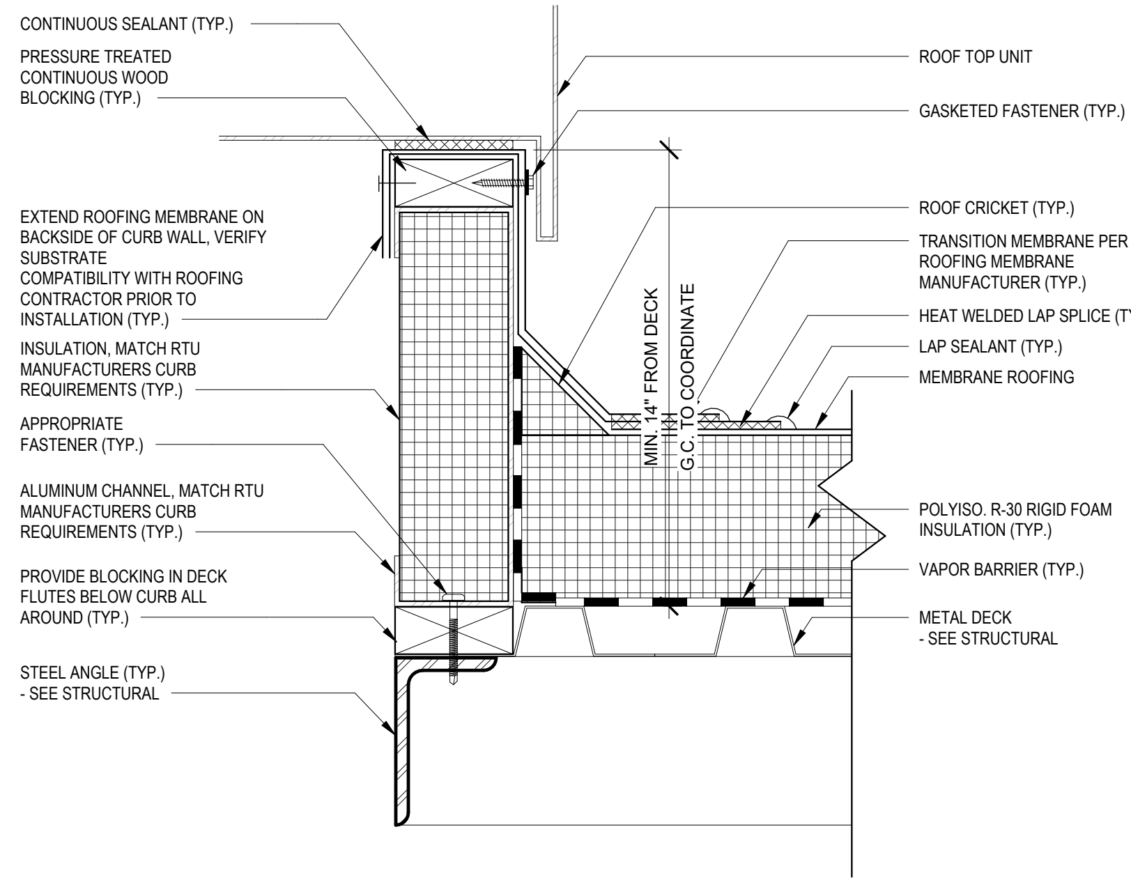
B4 ROOF CURB DETAIL 3" = 1'-0"
