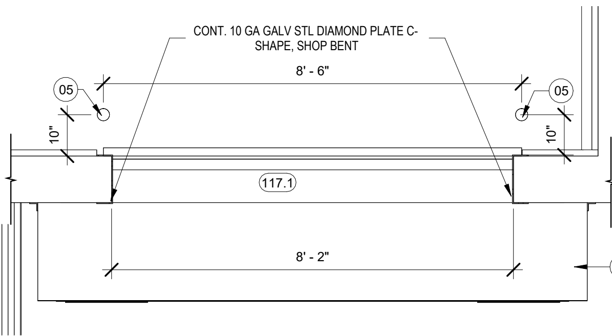
D5 DOCK DOOR - BOLLARDS 1/2" = 1'-0"
