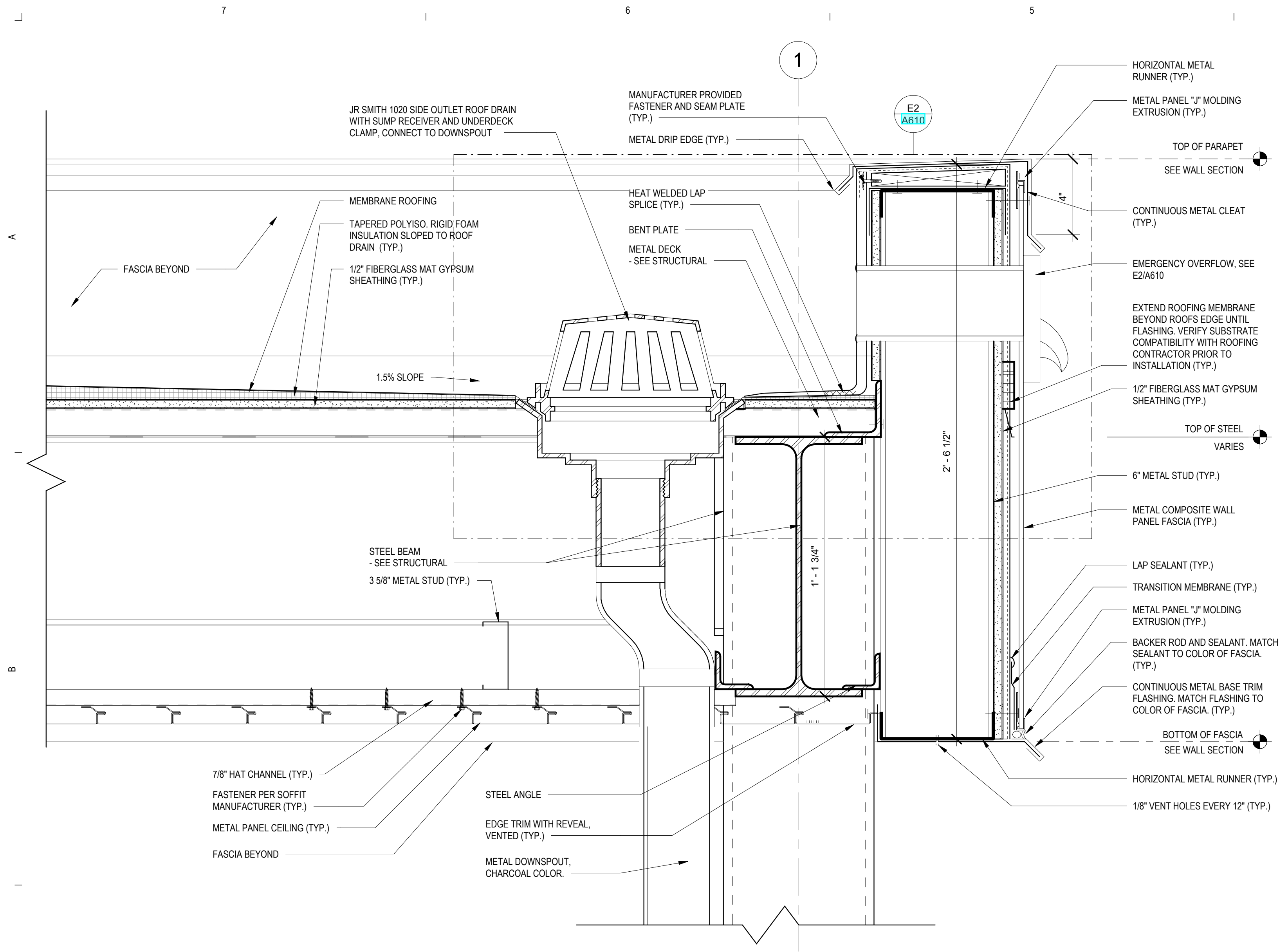
C6 CANOPY @ OUTSIDE EDGE 3" = 1'-0"
