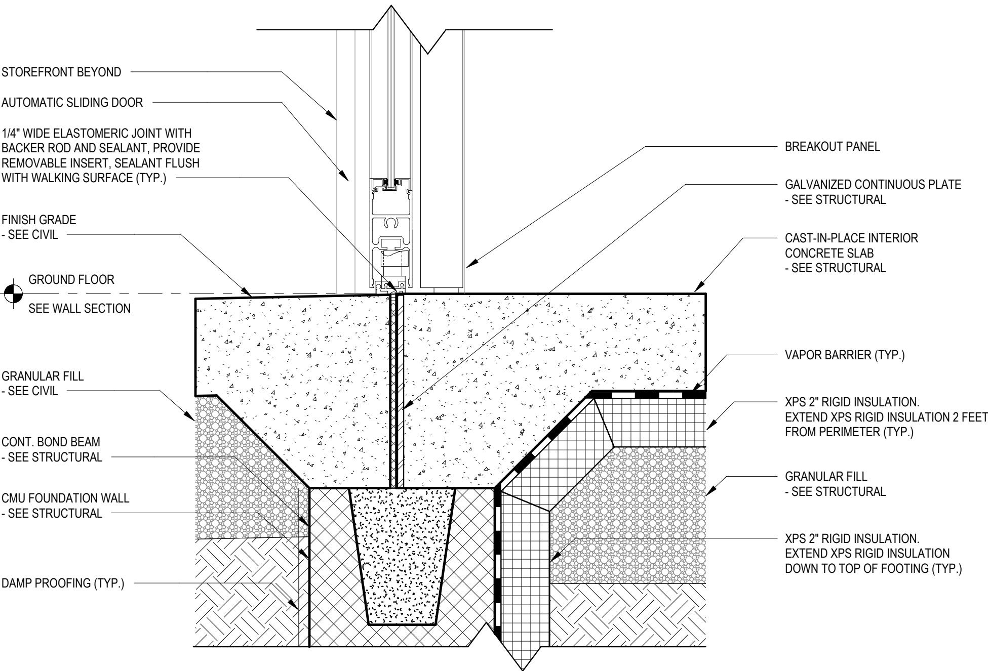
B4 SILL @ FRONT DOOR 3" = 1'-0"
