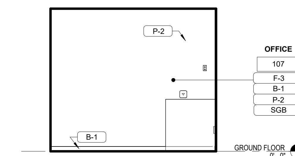
B1 INT ELEV - OFFICE 1/4" = 1'-0"
