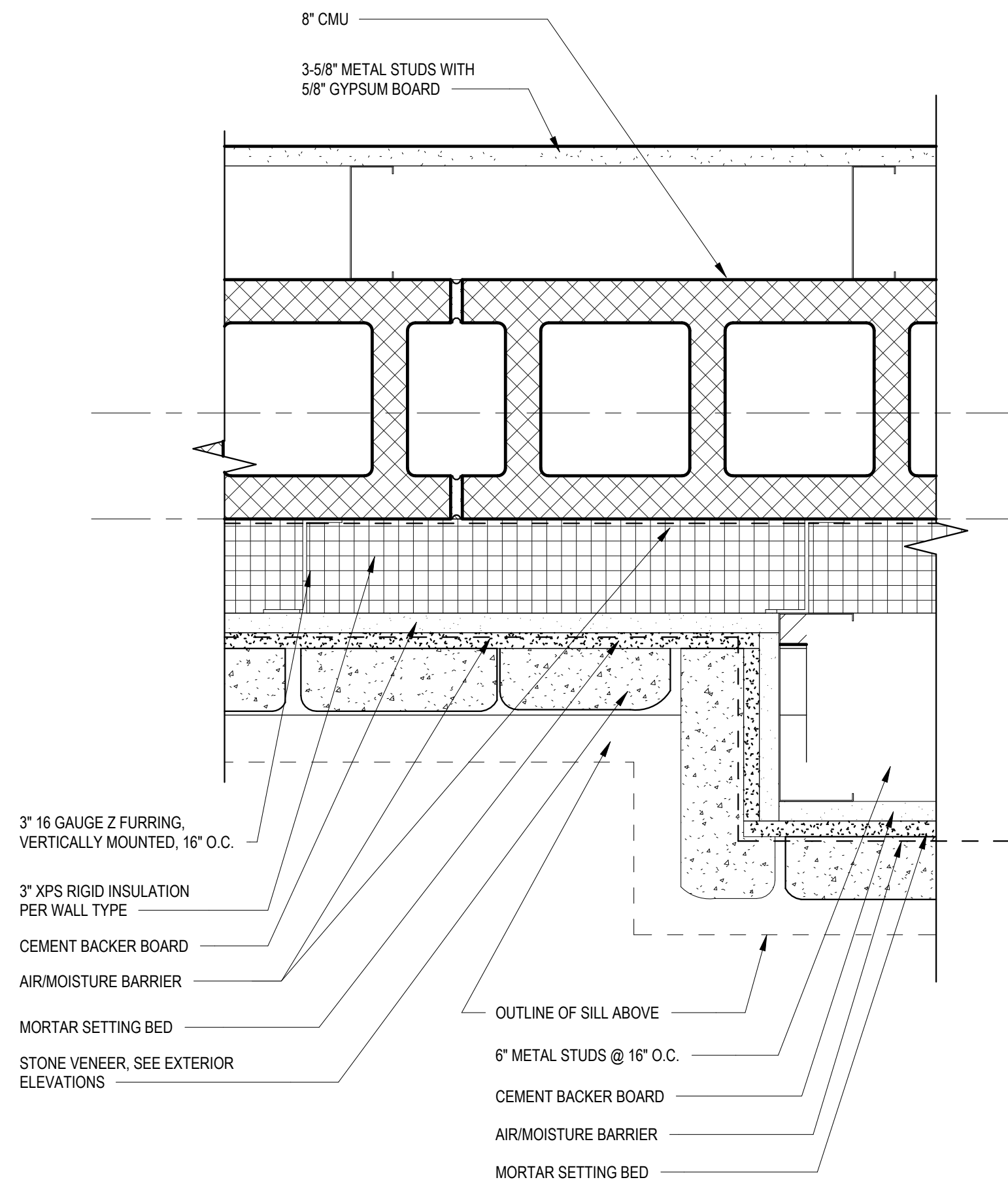
B4 BELOW WATER TABLE 3" = 1'-0"
