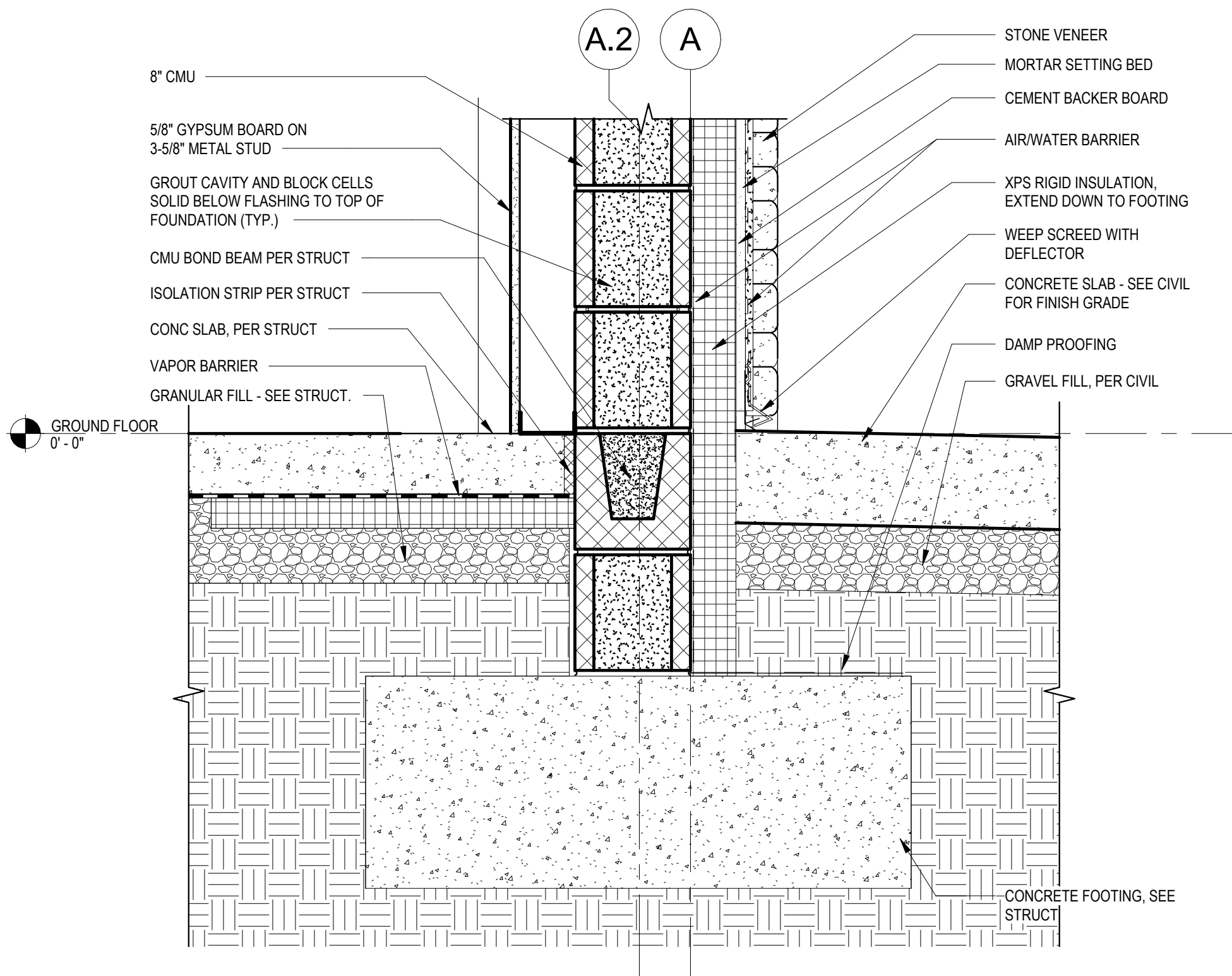
E4 FOUNDATION AT FRONT FACADE 1 1/2" = 1'-0"
