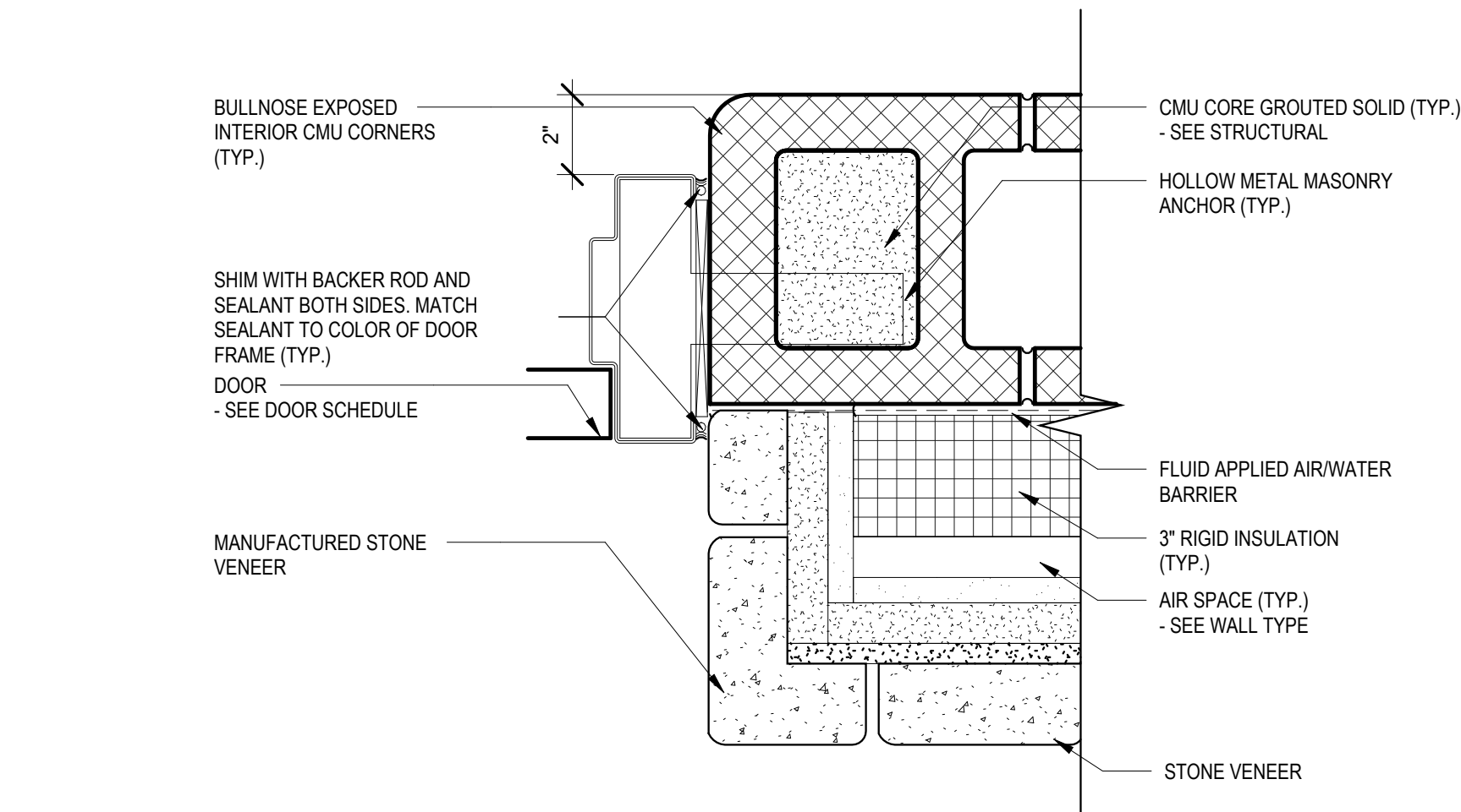
D2 EXTERIOR DOOR JAMB DETAIL - BELOW SILL 3" = 1'-0"
