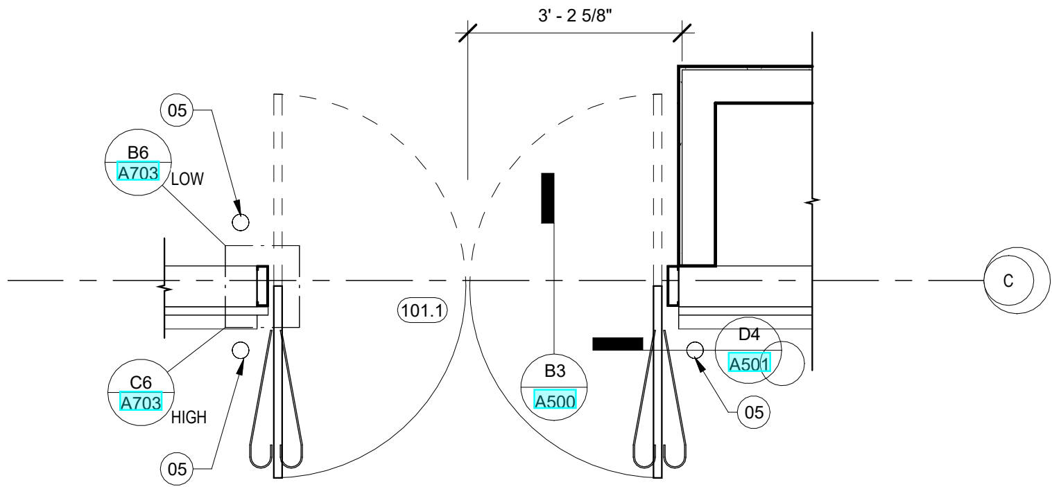
C5 TRAFFIC DOOR - BOLLARDS 1/2" = 1'-0"
