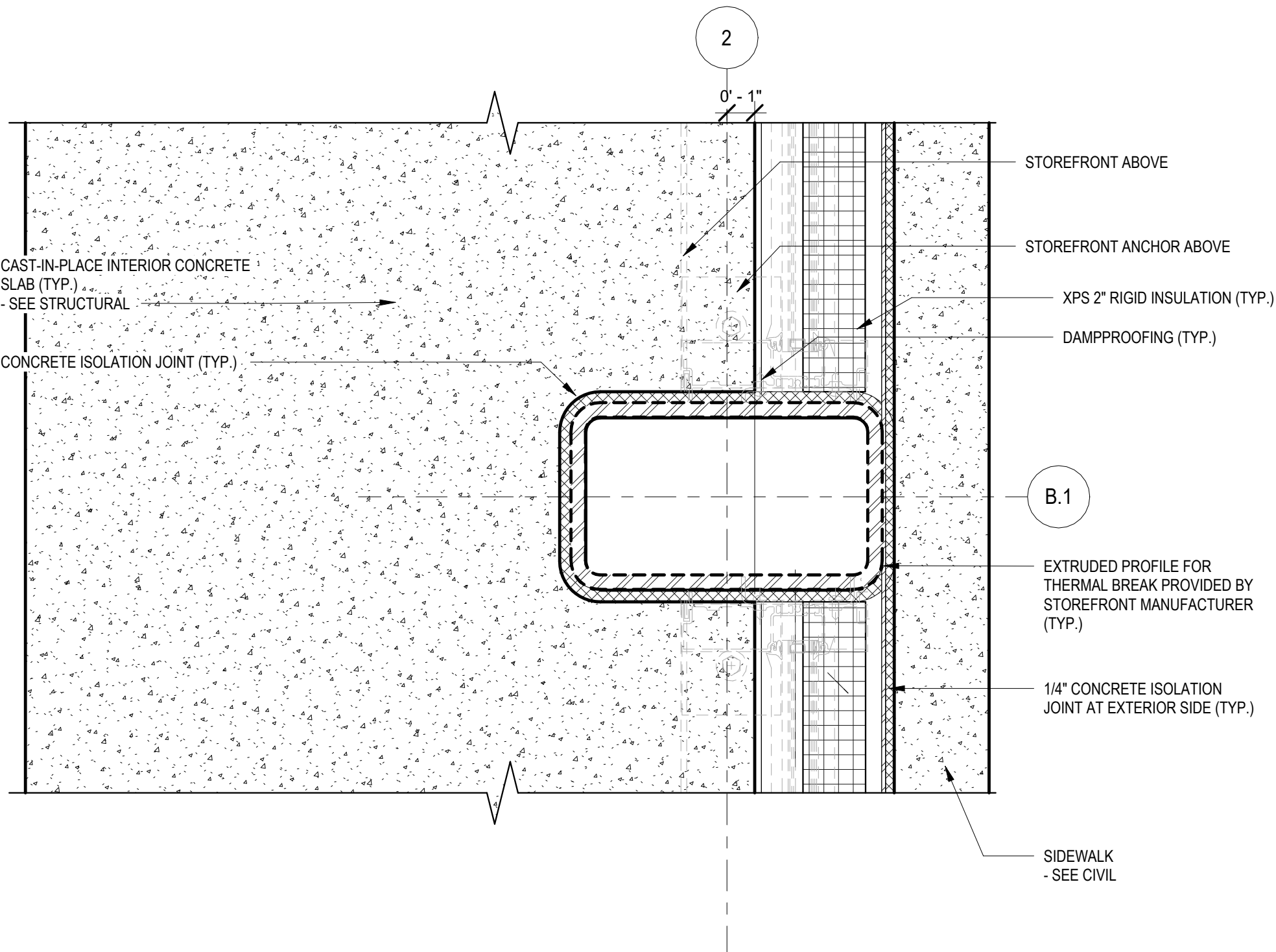
E6 THERMAL BREAK AT CORNER DETAIL 3" = 1'-0"
