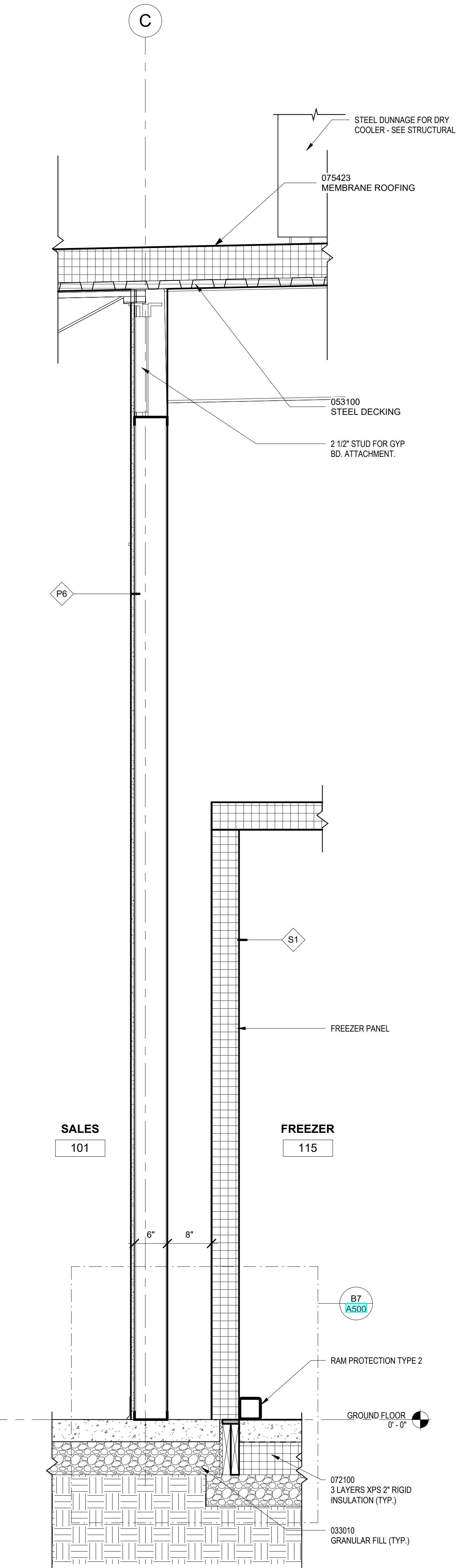
E6 INTERIOR WALL SECTION 1" = 1'-0"
