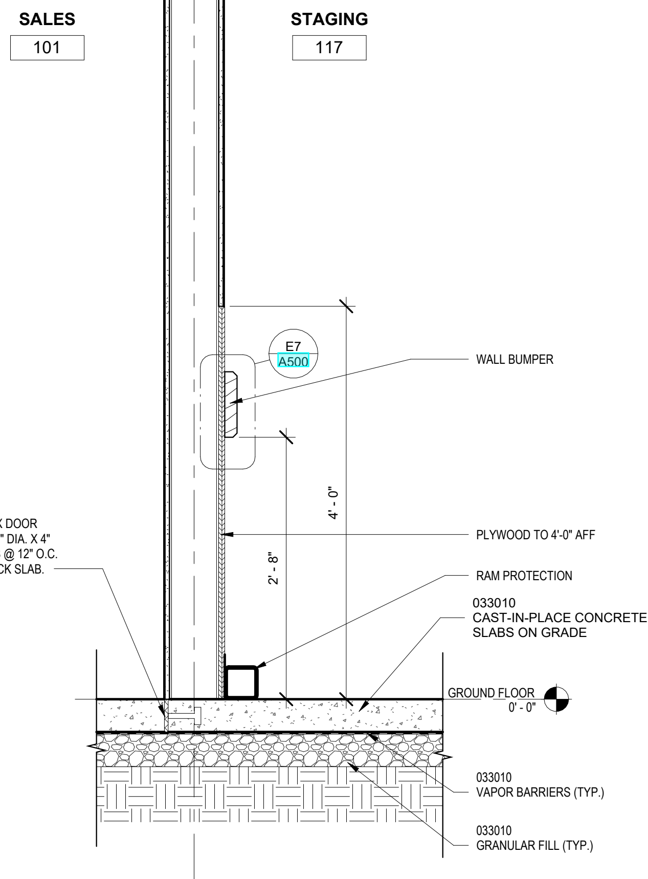
E7 WALL SECTION 1" = 1'-0"
