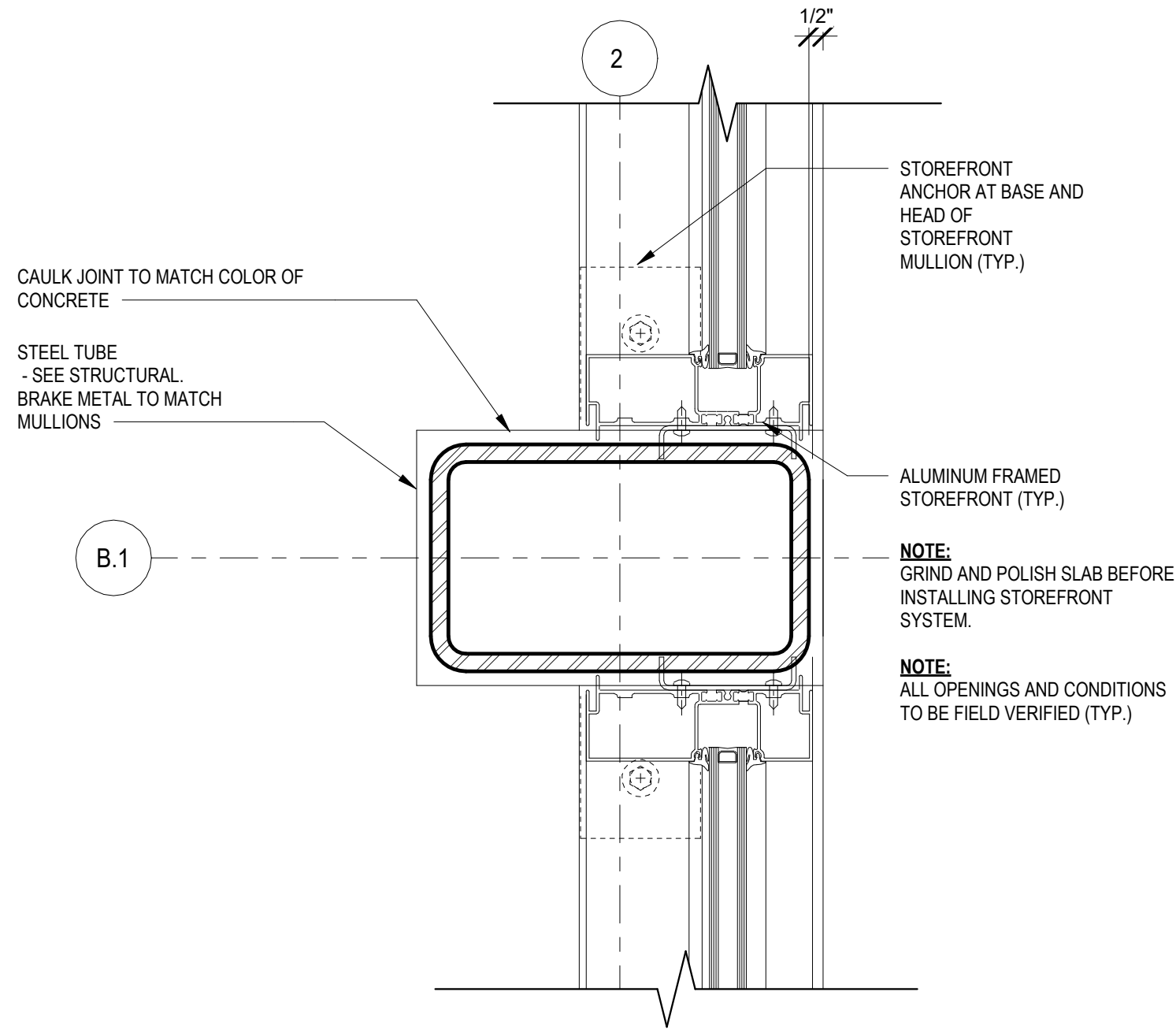
D6 COLUMN AT STOREFRONT 3" = 1'-0"
