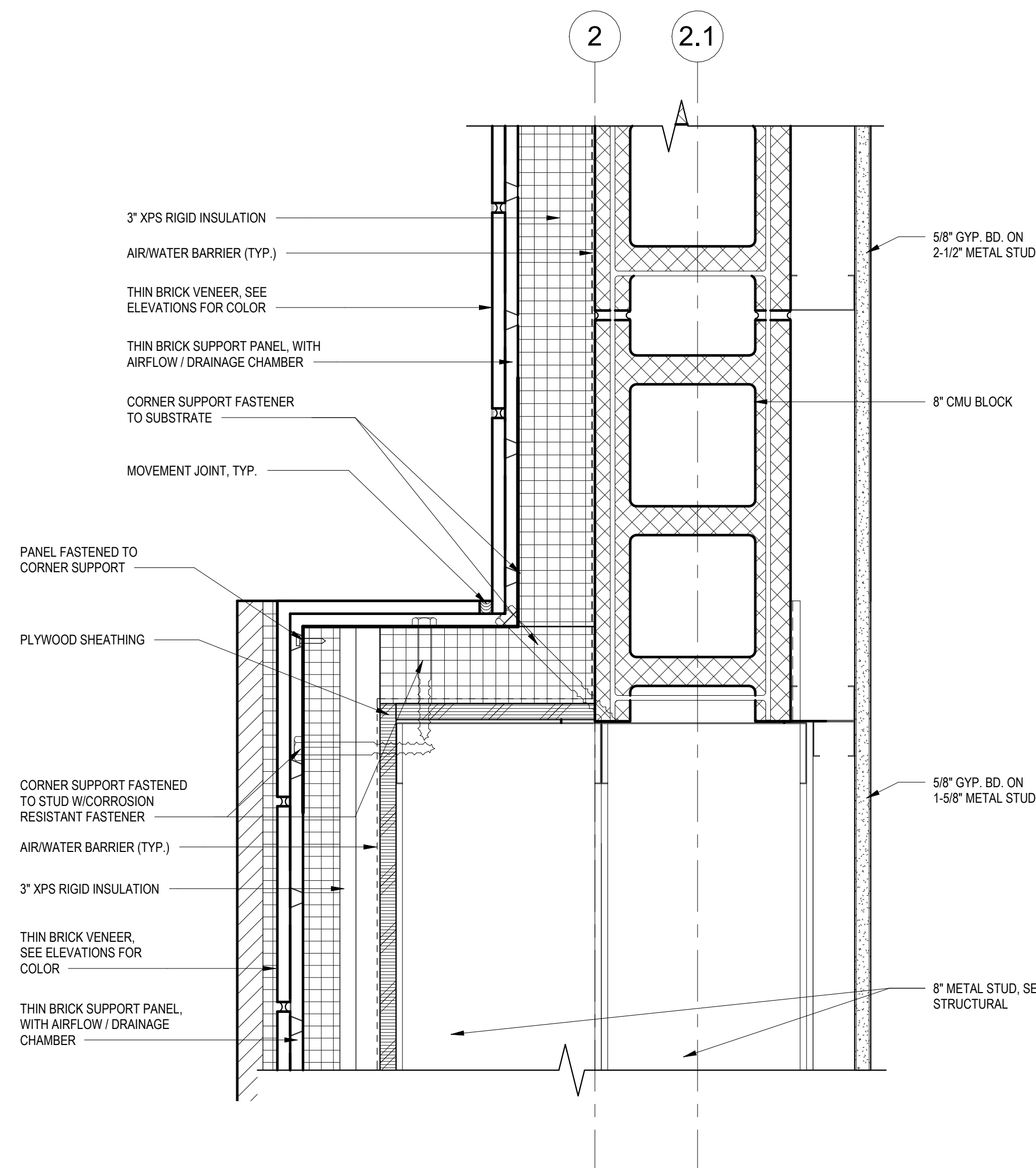
E2 SHEAR WALL TRANSITION ABOVE CANOPY 3" = 1'-0"
