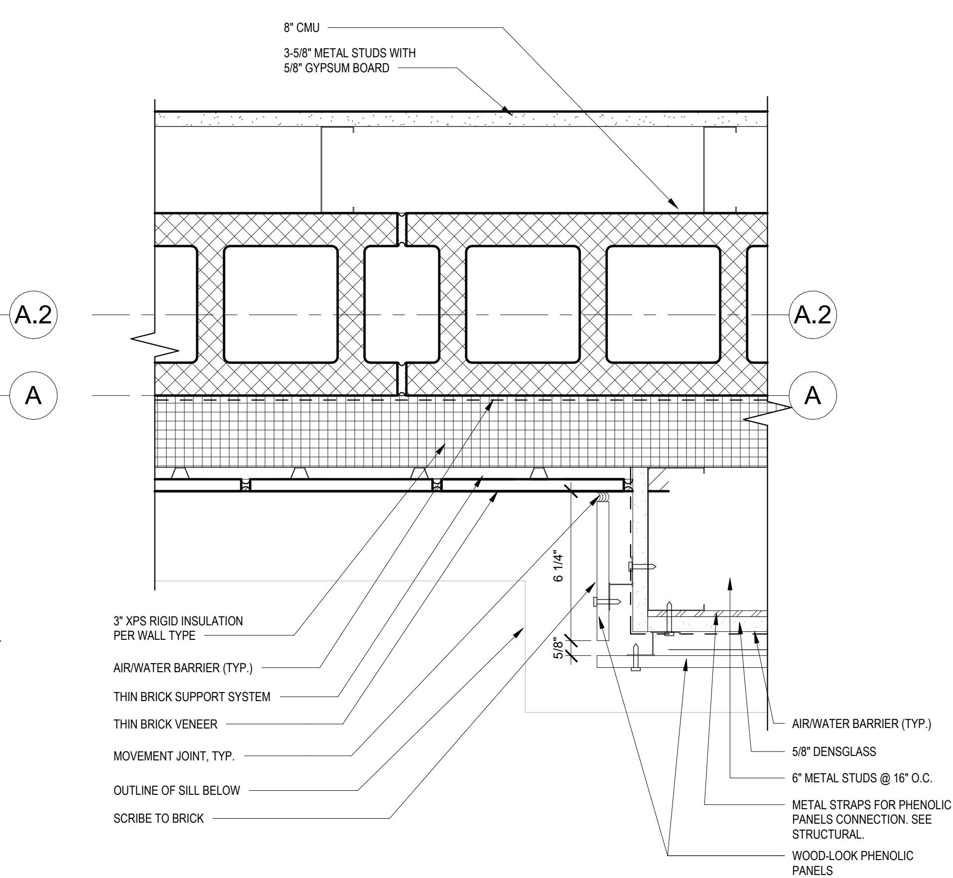
B2 FINISH TRANSITION SIDING TO BRICK 3" = 1'-0"
