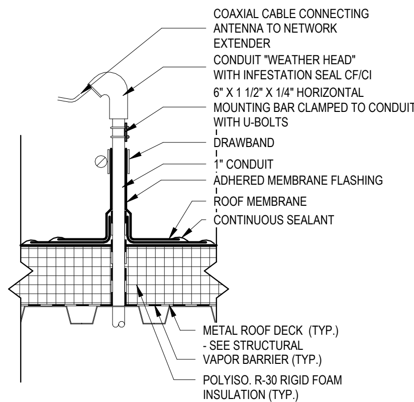
D4 GPS ANTENNA PENETRATION TYP. 1 1/2" = 1'-0"
