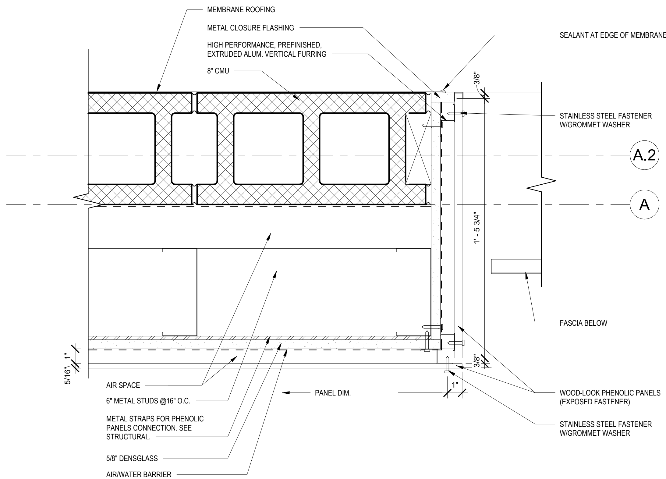
E6 PHENOLIC PANEL RETURN AT PARAPET 3" = 1'-0"
