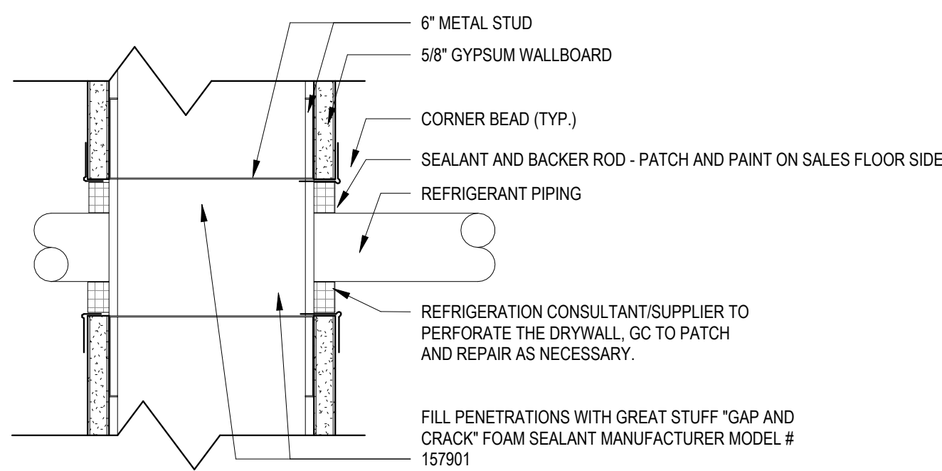
D5 PIPE PENETRATION BEHIND WALL FIXTURES 3" = 1'-0"
