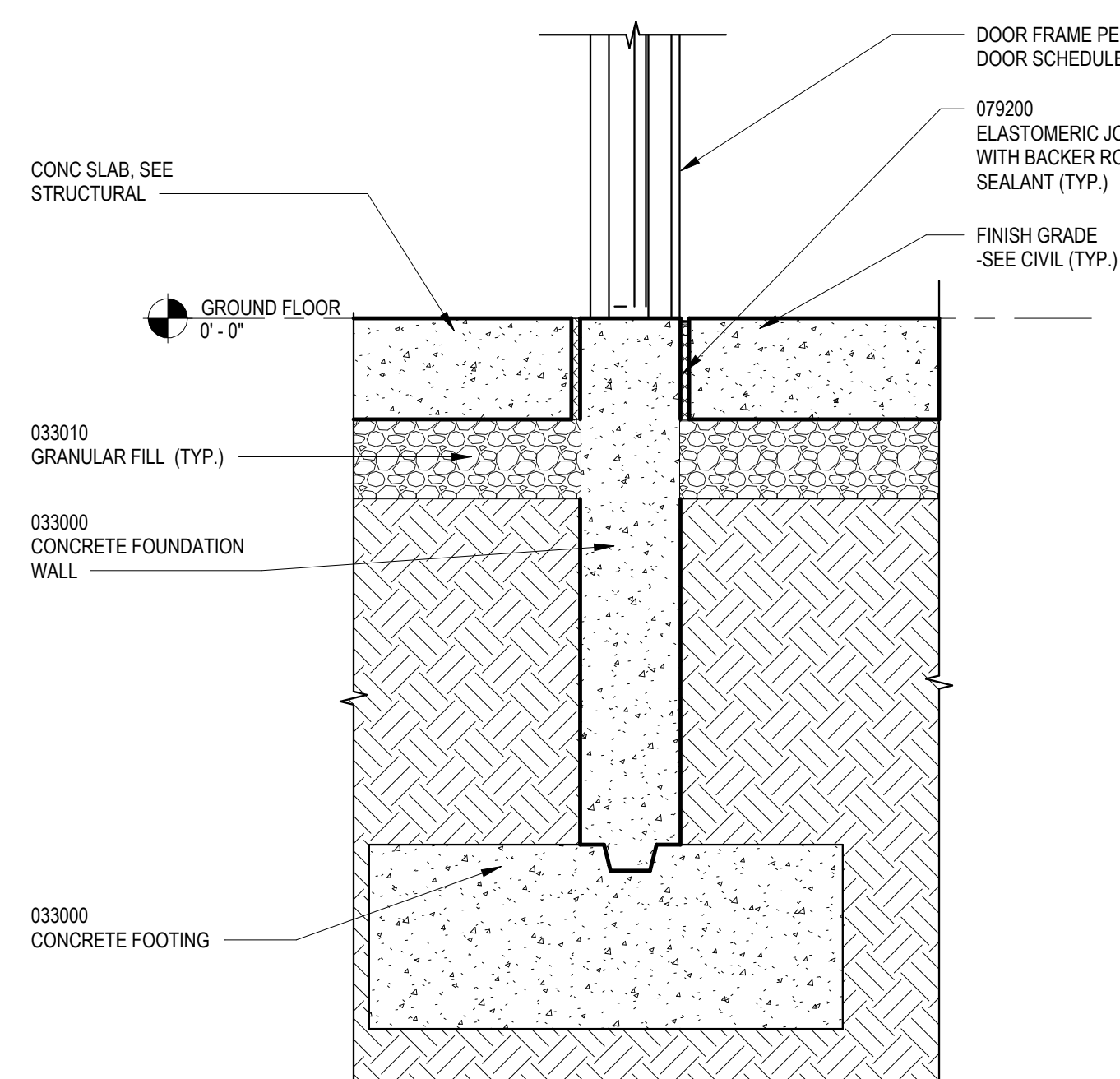
E2 FOUNDATION AT EXTERIOR DOOR 1" = 1'-0"
