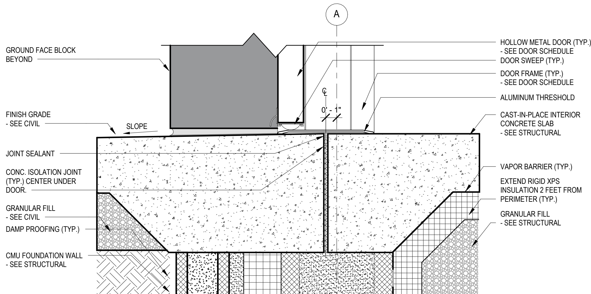
E2 EXTERIOR DOOR SILL DETAIL 3" = 1'-0"
