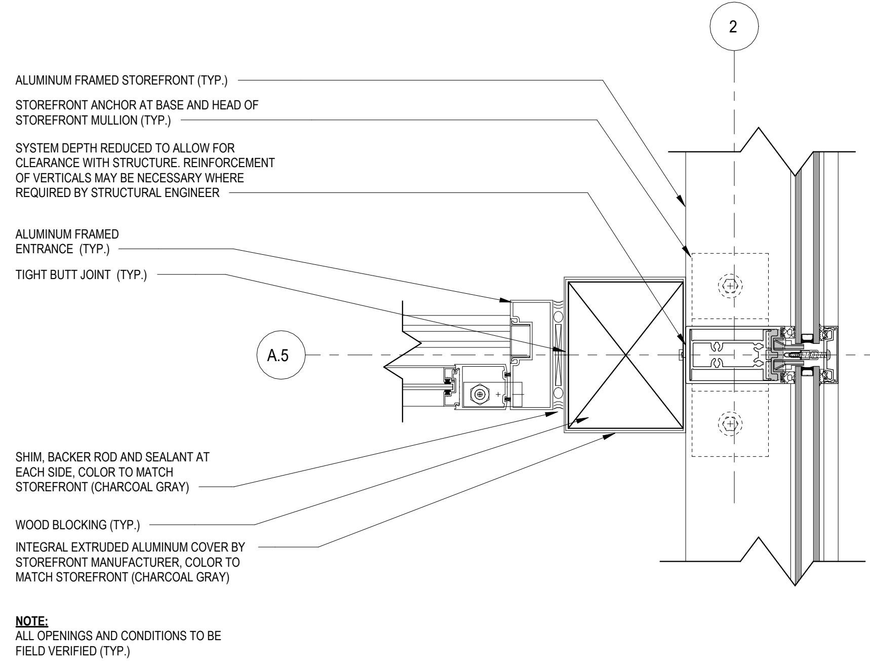
D4 VESTIBULE WALL @ STOREFRONT (TYP) 3" = 1'-0"
