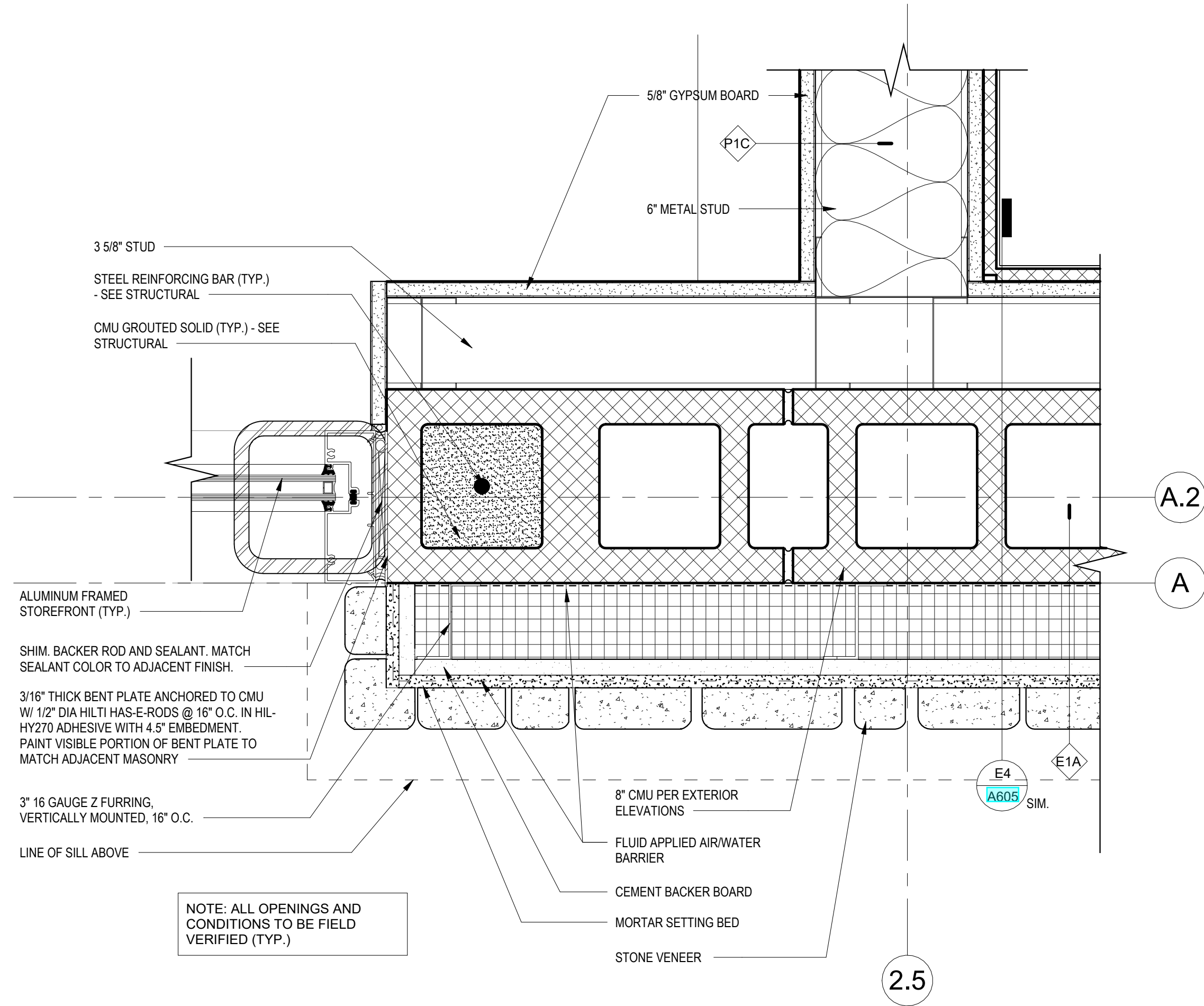
CORNER AT COLUMN LINE A-2.5 - BELOW WATER TABLE C6 3" = 1'-0"
