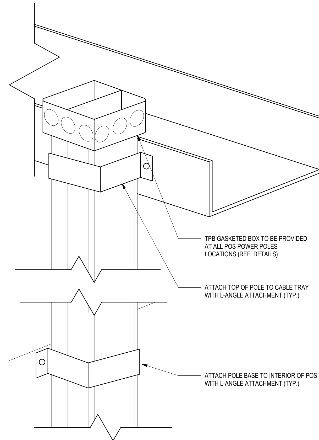
D3 POS POWER POLE 1/2" = 1'-0"
