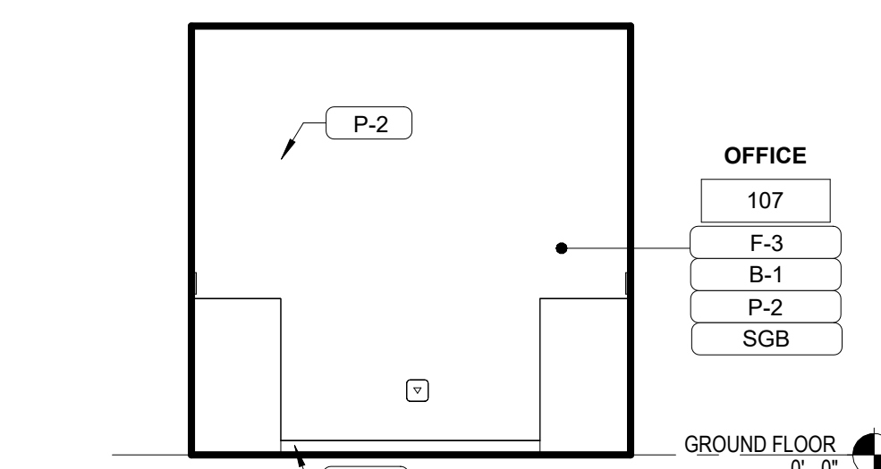
B2 INT ELEV - OFFICE 1/4" = 1'-0"
