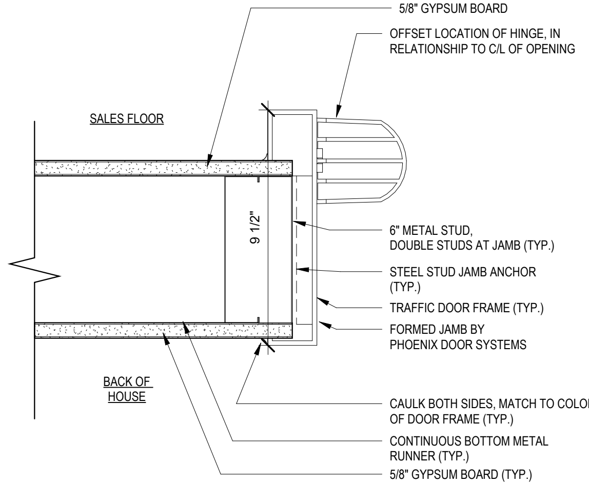
C6 TRAFFIC DOOR JAMB DETAIL - HIGH 3" = 1'-0"
