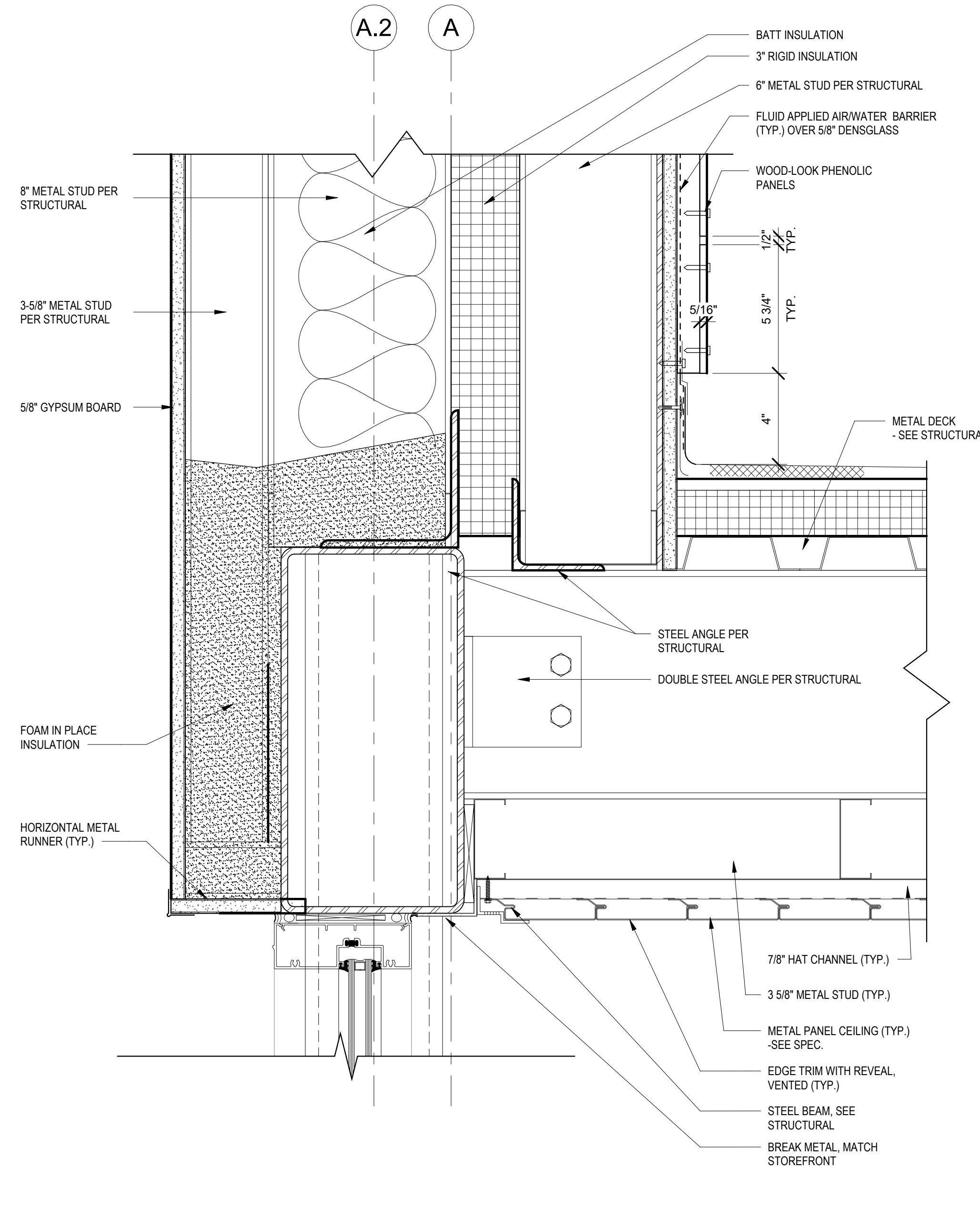
E4 CANOPY TO WALL CONNECTION AT SIDING 3" = 1'-0"
