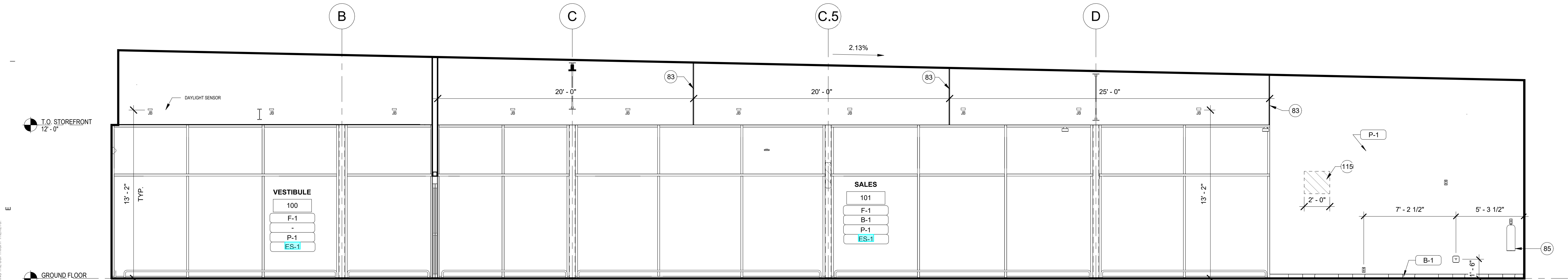
E7 INTERIOR ELEVATION - SALES FLOOR 1/4" = 1'-0"
