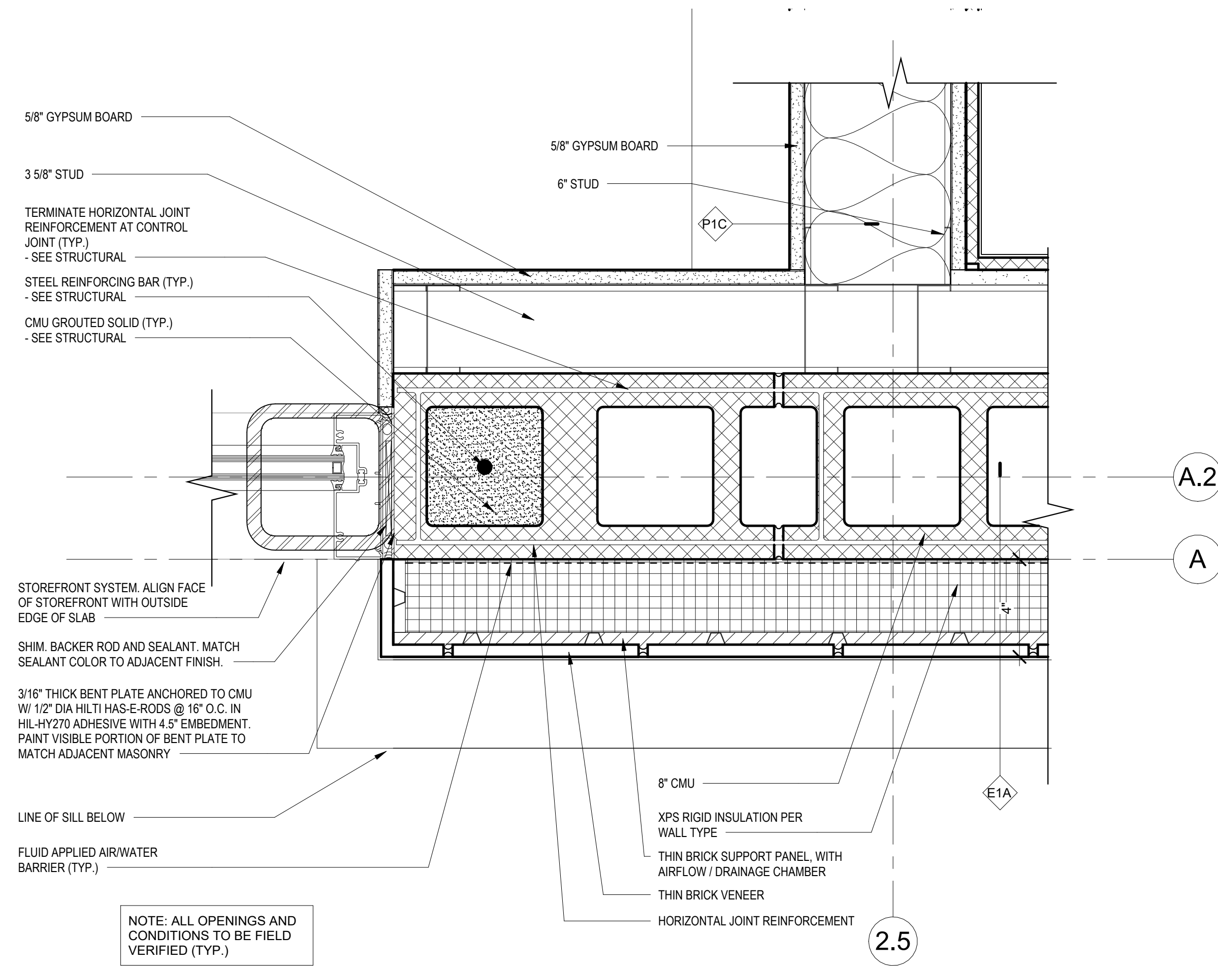
CORNER AT COLUMN LINE A-2.5 - ABOVE WATER TABLE C2 3" = 1'-0"
