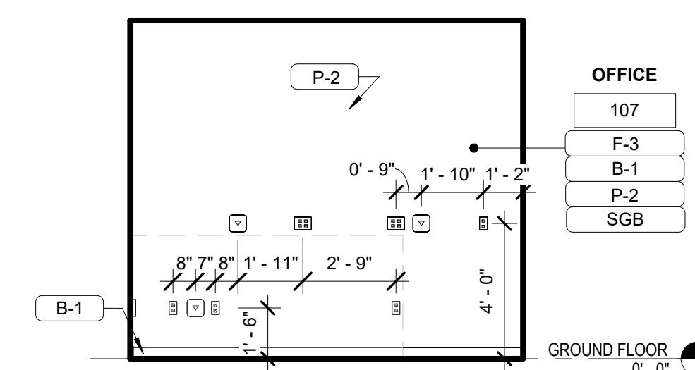
C2 INT ELEV - OFFICE 1/4" = 1'-0"
