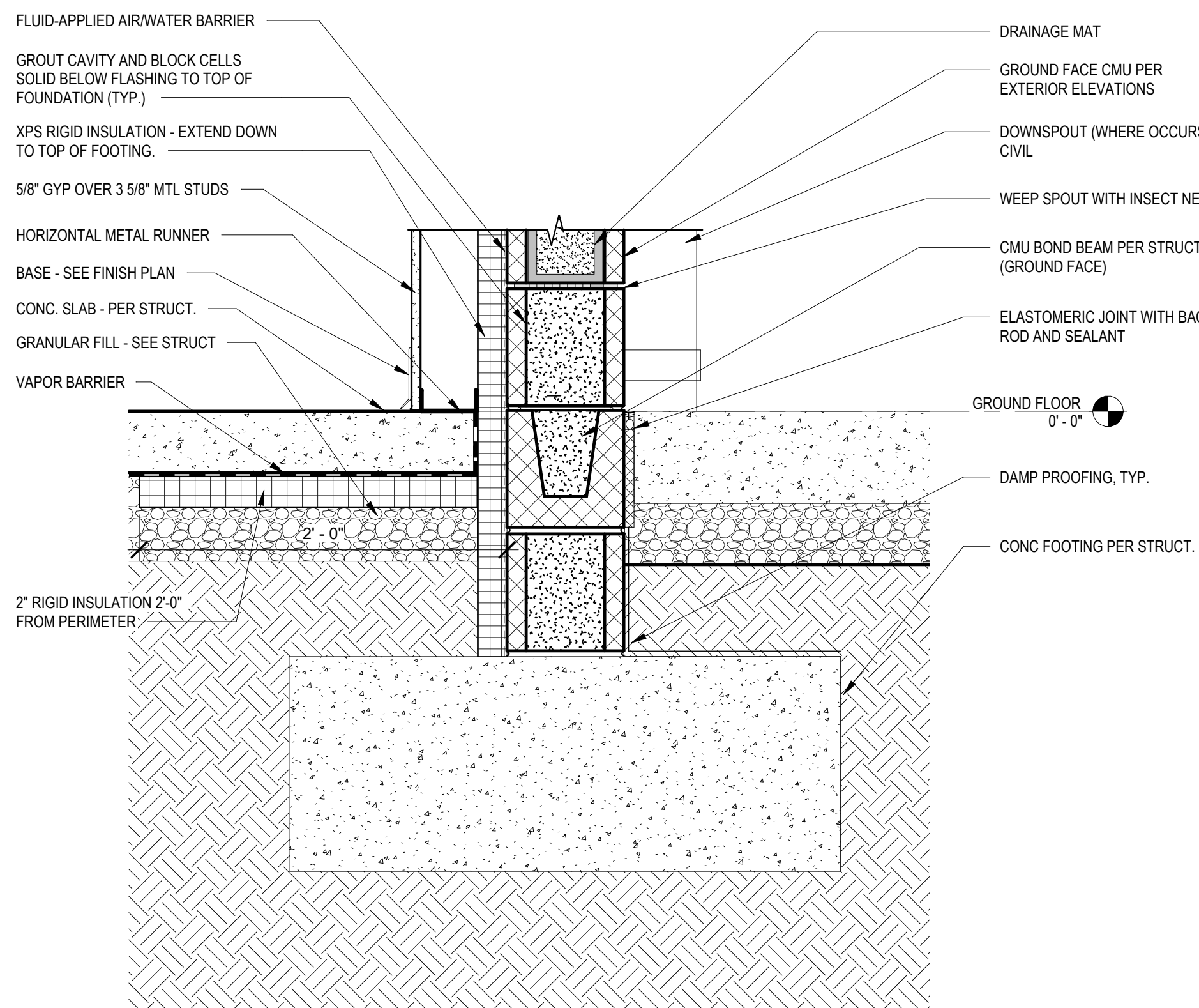
D4 FOUNDATION AT BACK WALL 1 1/2" = 1'-0"
